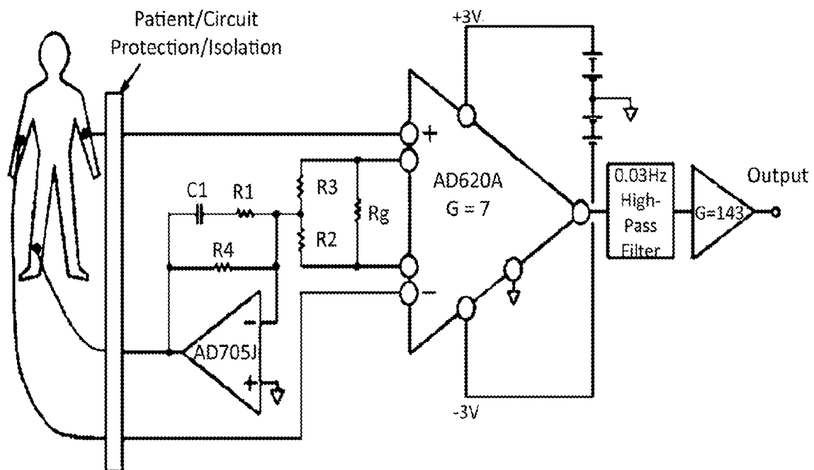
Fig. 12 Prior Art
