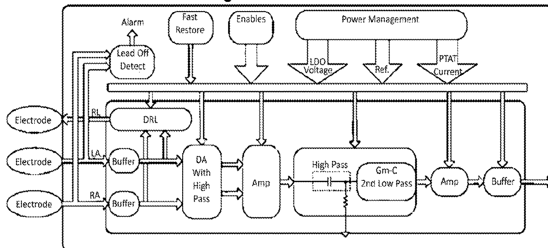
Fig. 16 Prior Art
