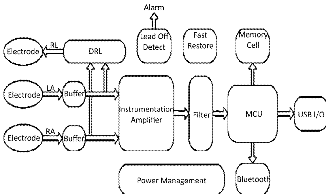
Fig. 15 Prior Art
