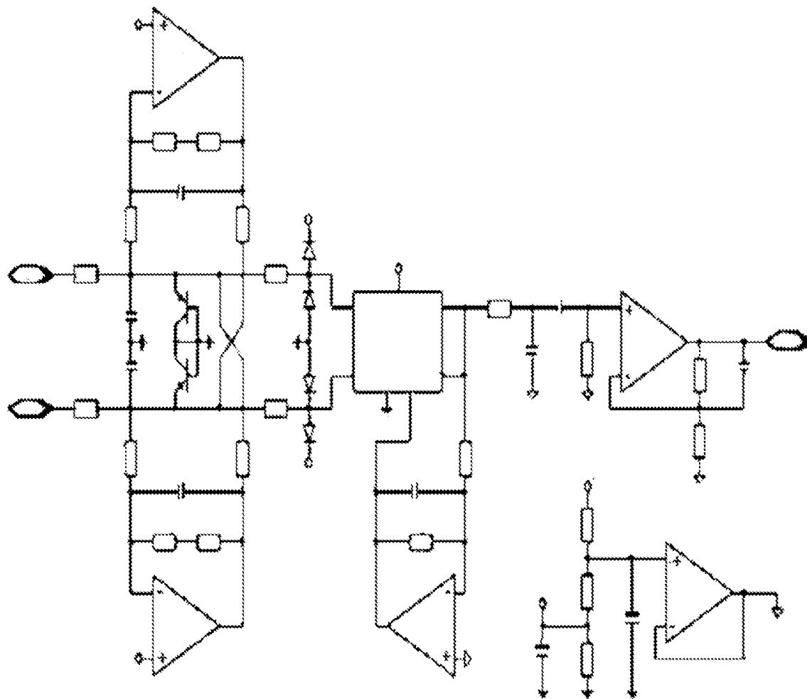
Fig. 13 Prior Art
