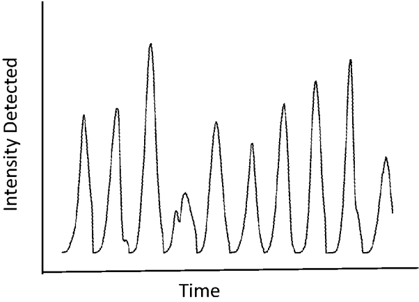
603 Result of Multiplying Reflected Electronic Signal Intensity for \lambda_1 and Doppler Signal Synchronized Over Time
