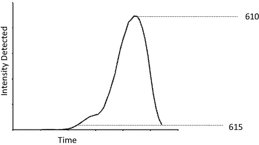
604 Result of Multiplying Reflected Electronic Signal Intensity for \lambda_1 and Doppler Signal Synchronized Over Time (Averaged Over Several Periods)
