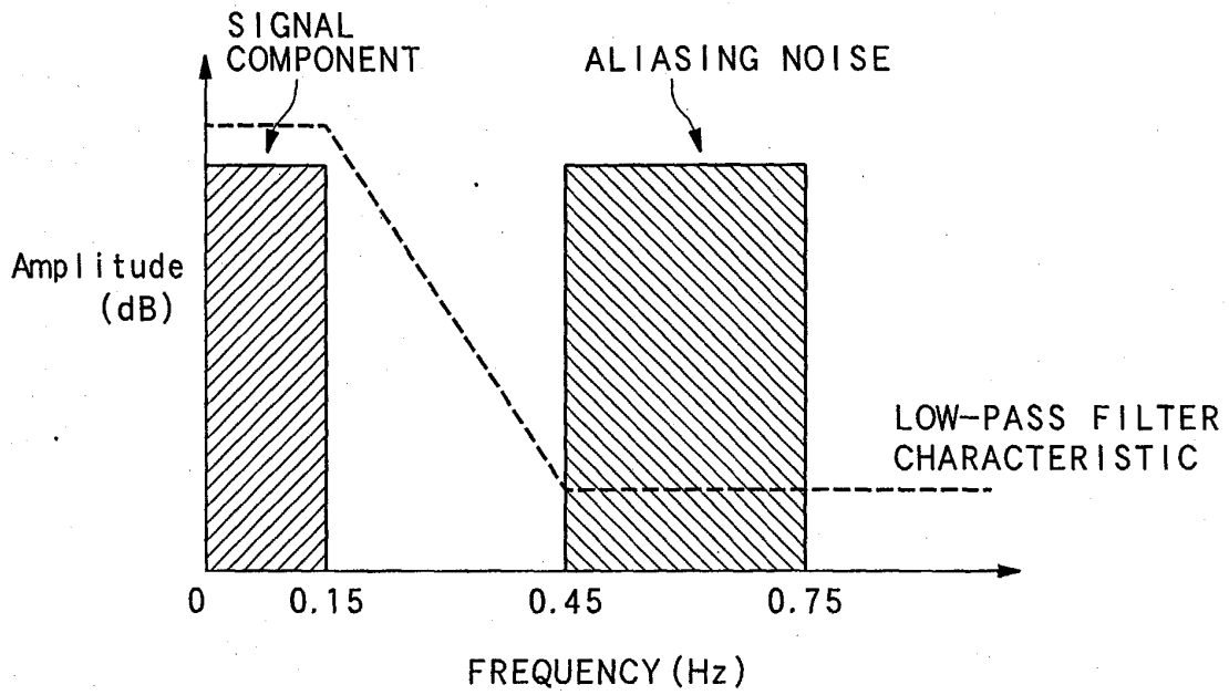
FIG. 3 PRIOR ART
