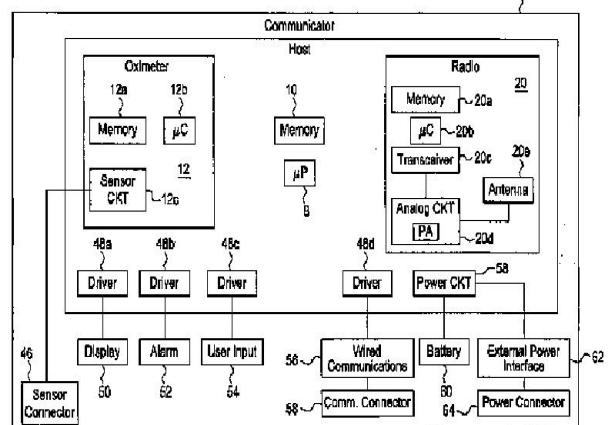
FIG. 13 Communicator Block Diagram
