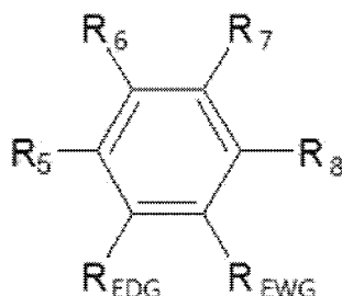
[Chemical Formula 1]
