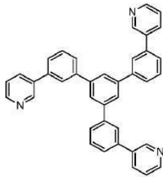
TmPyPb
