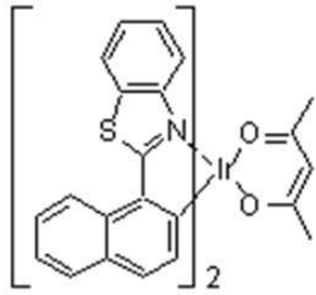
\alpha bsn 2 Ir(acac) (602nm)
