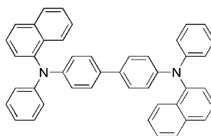
NPB
