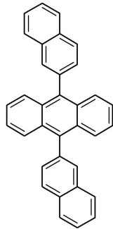
AND 9,10-di(2-naphthyl)anthracene
