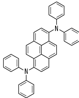
1,6-Bis(diphenylamine)pyrene
