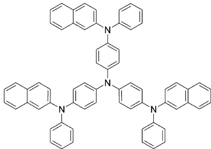
2-TNATA
