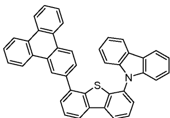
Compound E26
