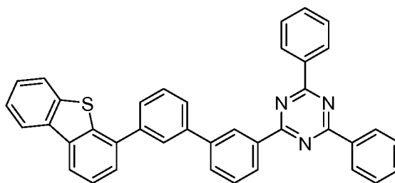
Compound D3
