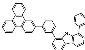
Compound E8
