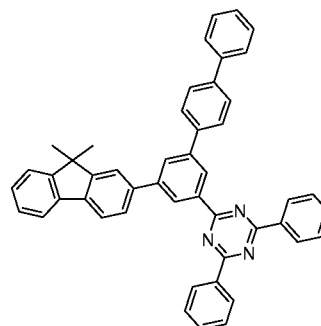
Compound B3
