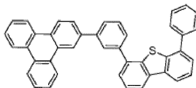
(Composé E8,
