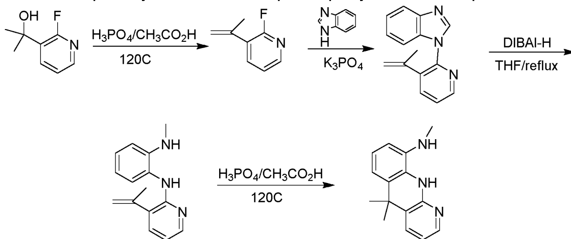
Scheme 1: Proposed synthesis of metal complex via phenylenediamine compound of Formula 1
