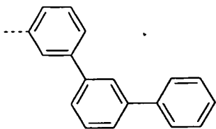
formula (15)
