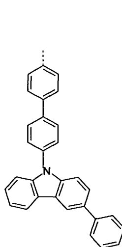
formula (61)
