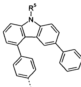
formula (66)
