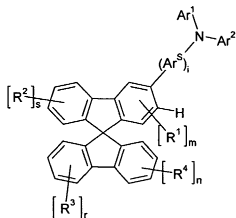
formula (5)
