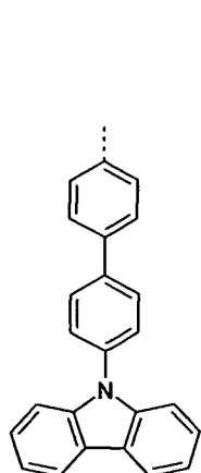
formula (59)
