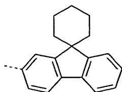
formula (20d)
