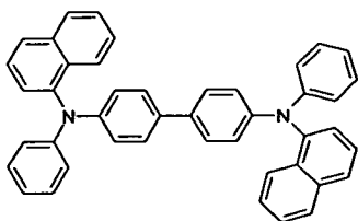
NPB
