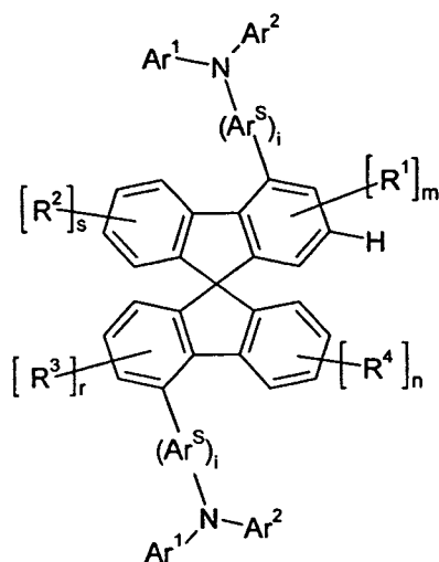
formula (3)
