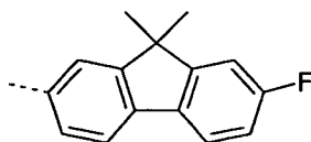
formula (20e)
