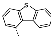
formula (35)
