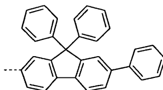
formula (20i)
