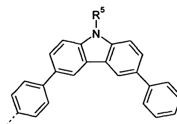
formula (64)
