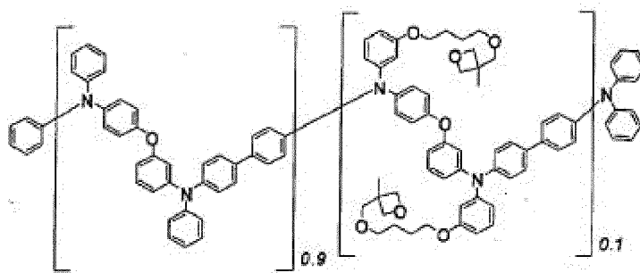
(Target compound 29)
