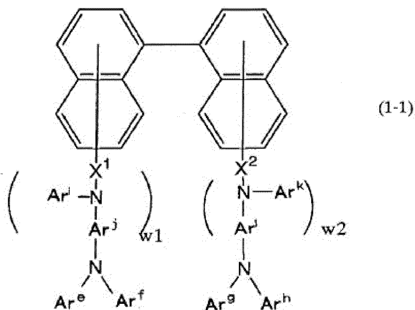
[Formula 43]
