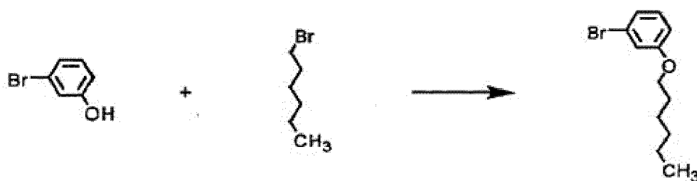
(Target compound 13)
