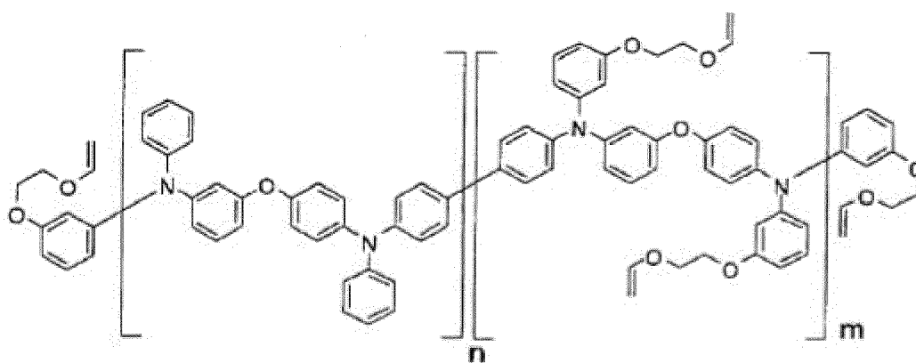
[Formula 34]
