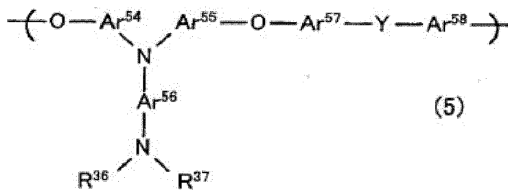
[Formula 47]
