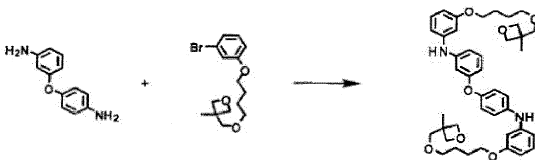
(Target compound 2)
