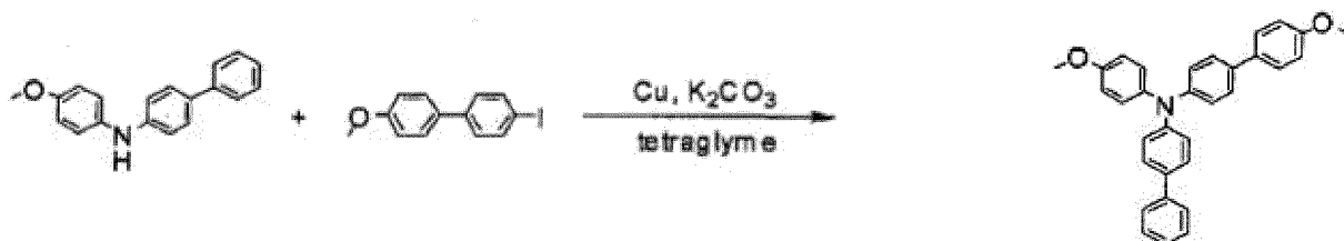
Target compound 4
