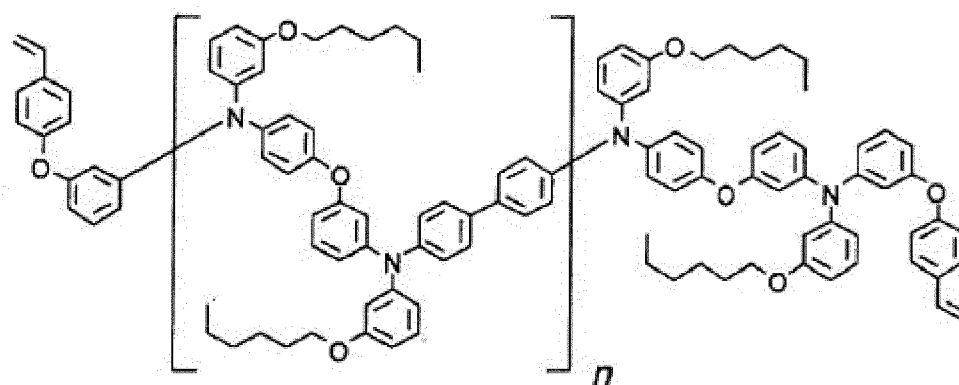
[Formula 33]
