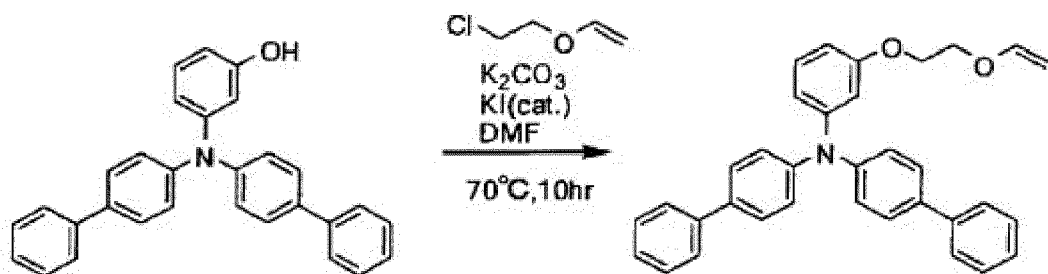
(Target compound 22)
