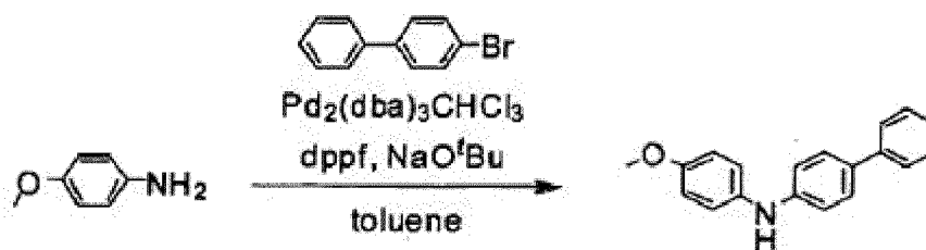
Target compound 4
