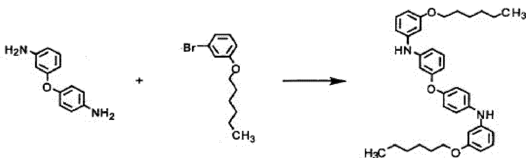
(Target compound 13)
