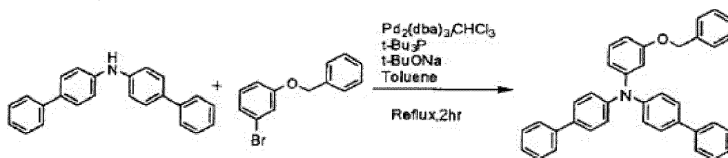
(Target compound 21)
