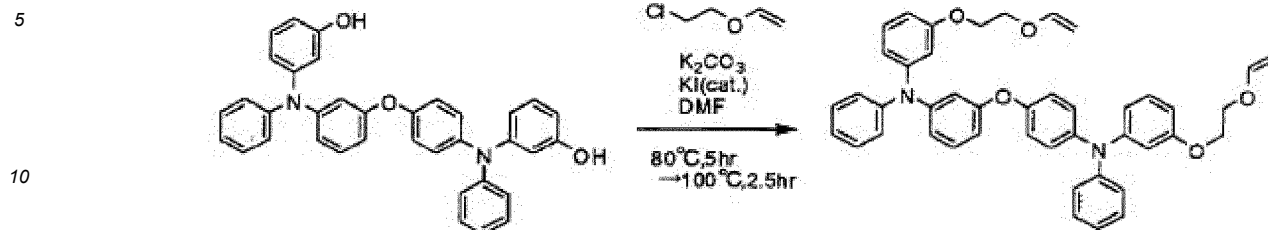
Target compound 26
