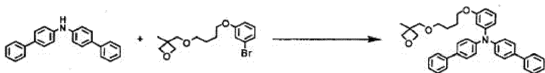
Target compound 2
