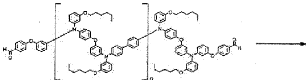
(Target compound 15)
