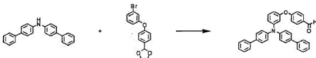
(Intermediate 1)
