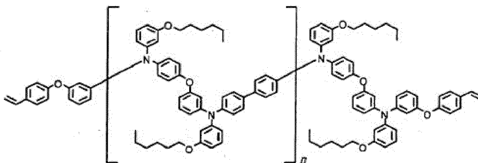
(Target compound 16)
