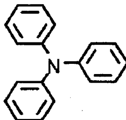
[Formula 9]
