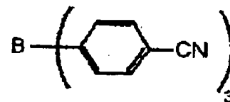
6-9
