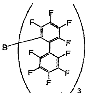
6-16
