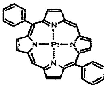
(D-5)
