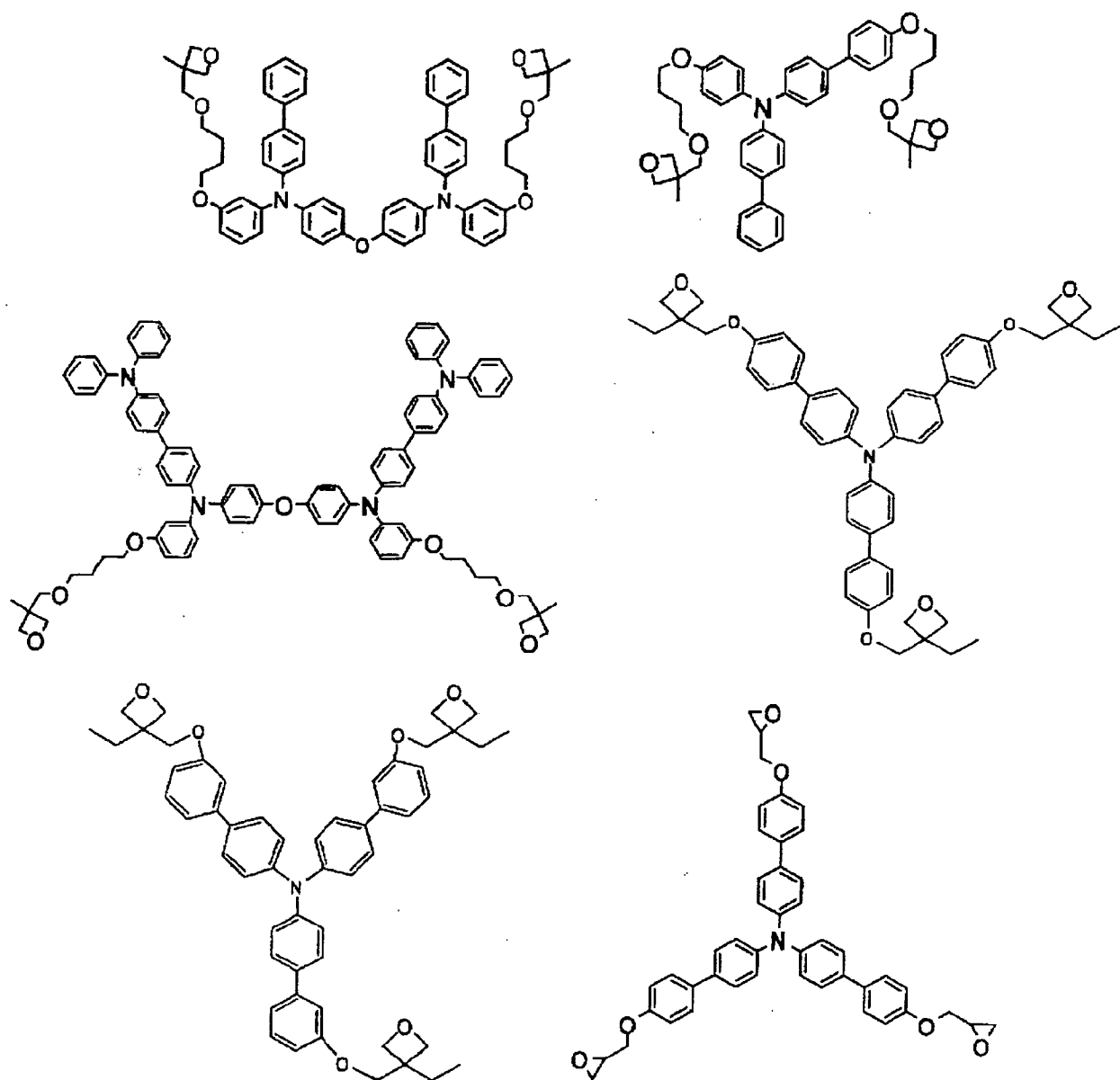
[Formula 30]
