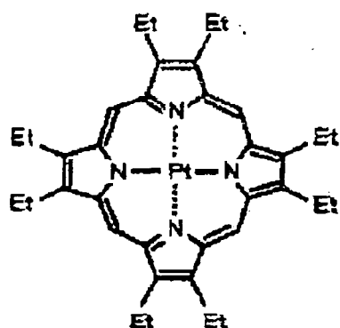
(D-1)
