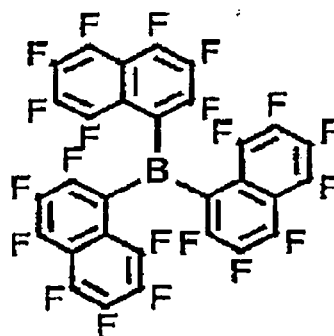
6-17
