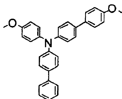
Target compound 6
