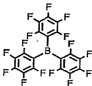
[Formula 53]
