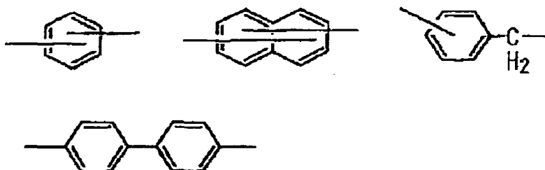
[Formula 42]
