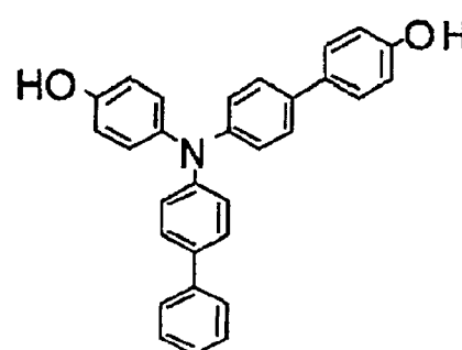
Target compound 7
