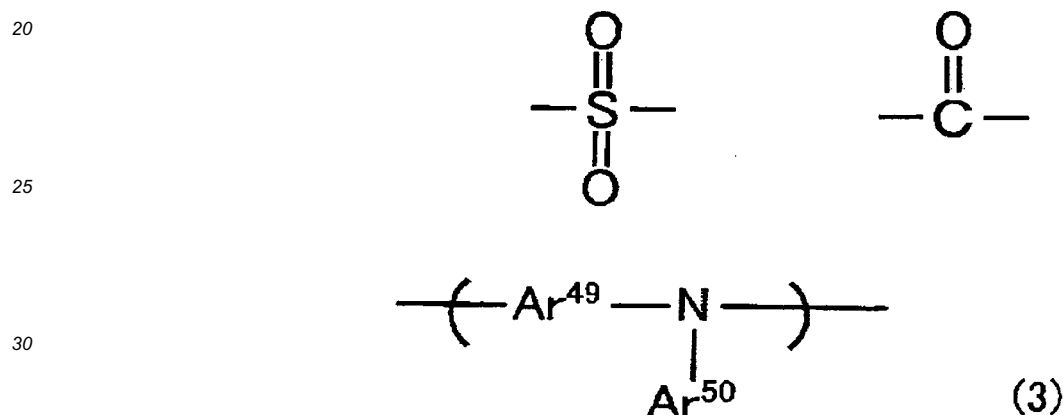
[Formula 45]
