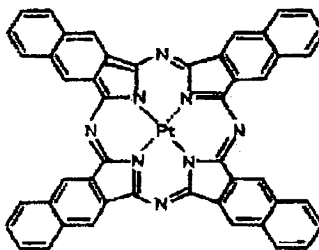
(D-7)
