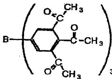
6-11
