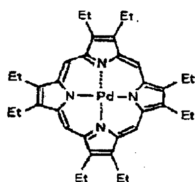
(D-3)
