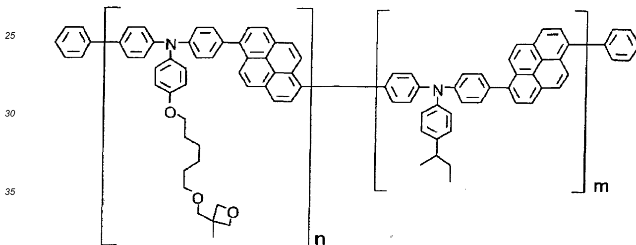
[Formula 39]
