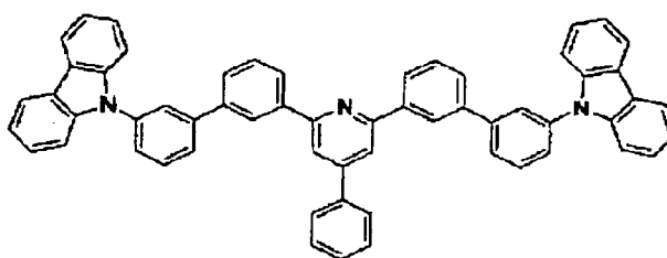
(C1)
