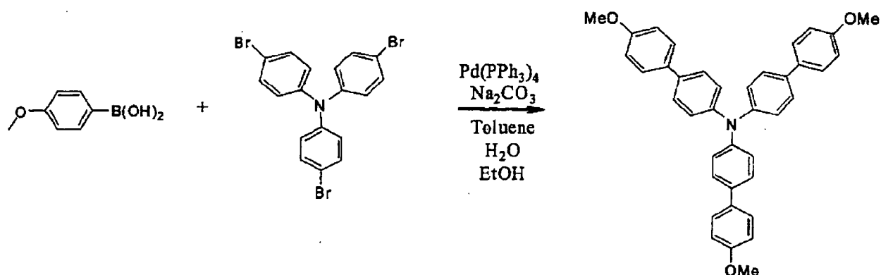
(Target compound 9)
