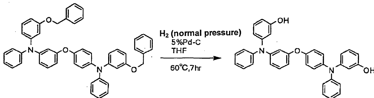
Target compound 25
