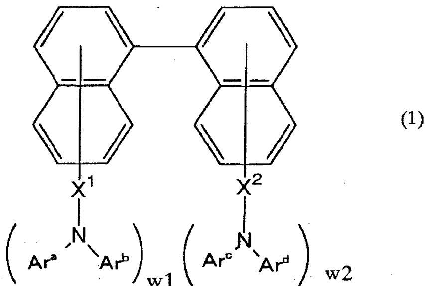
[Formula 41]
