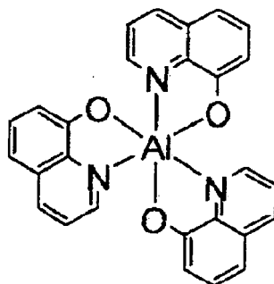
(C5)
