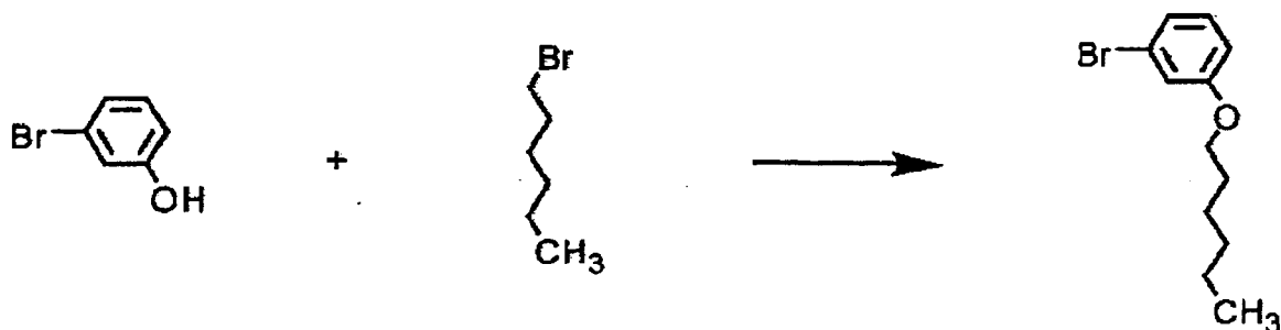
(Target compound 13)
