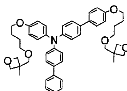
Target compound 8
