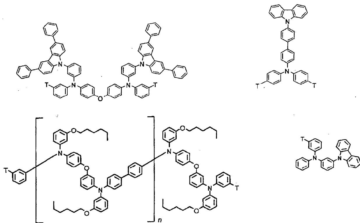
[Formula 29]
