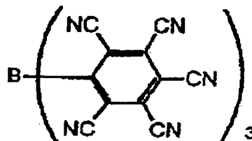
6-5
