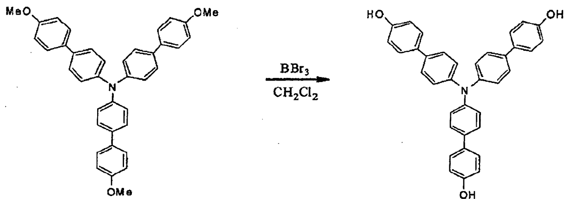
(Target compound 10)
