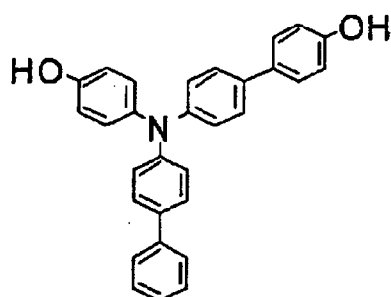
Target compound 7
