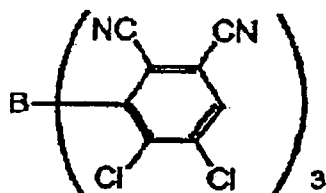
6-7
