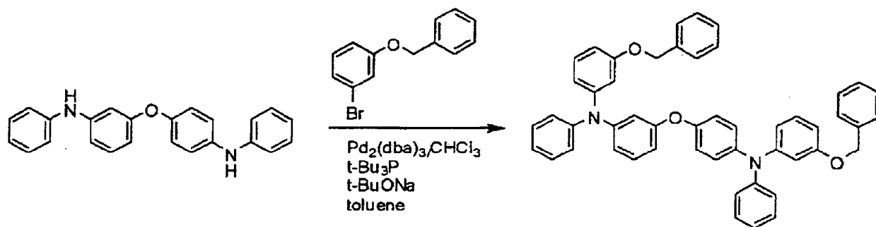
Target compound 24
