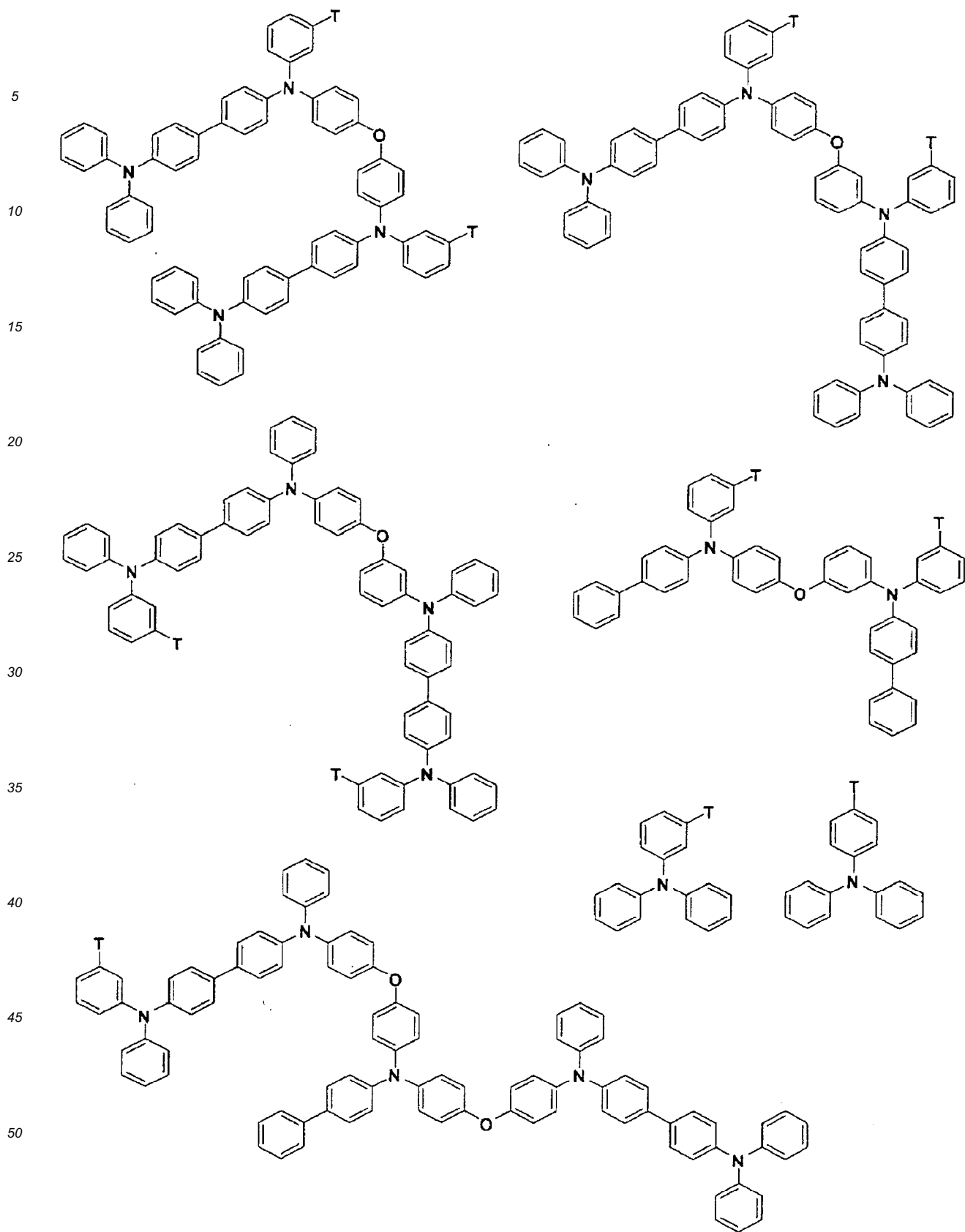
[Formula 19]
