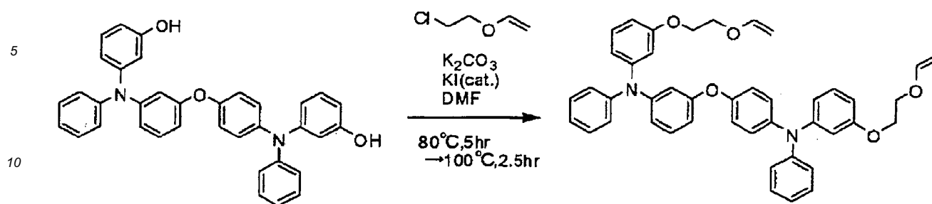
Target compound 26
