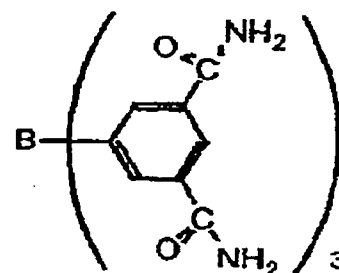
6-12
