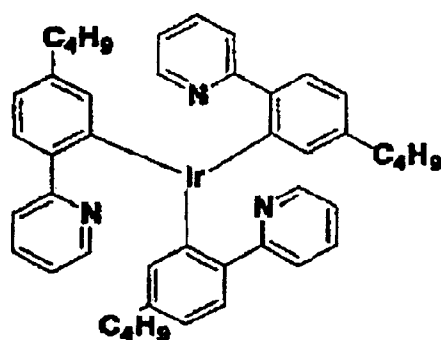
(C3)
