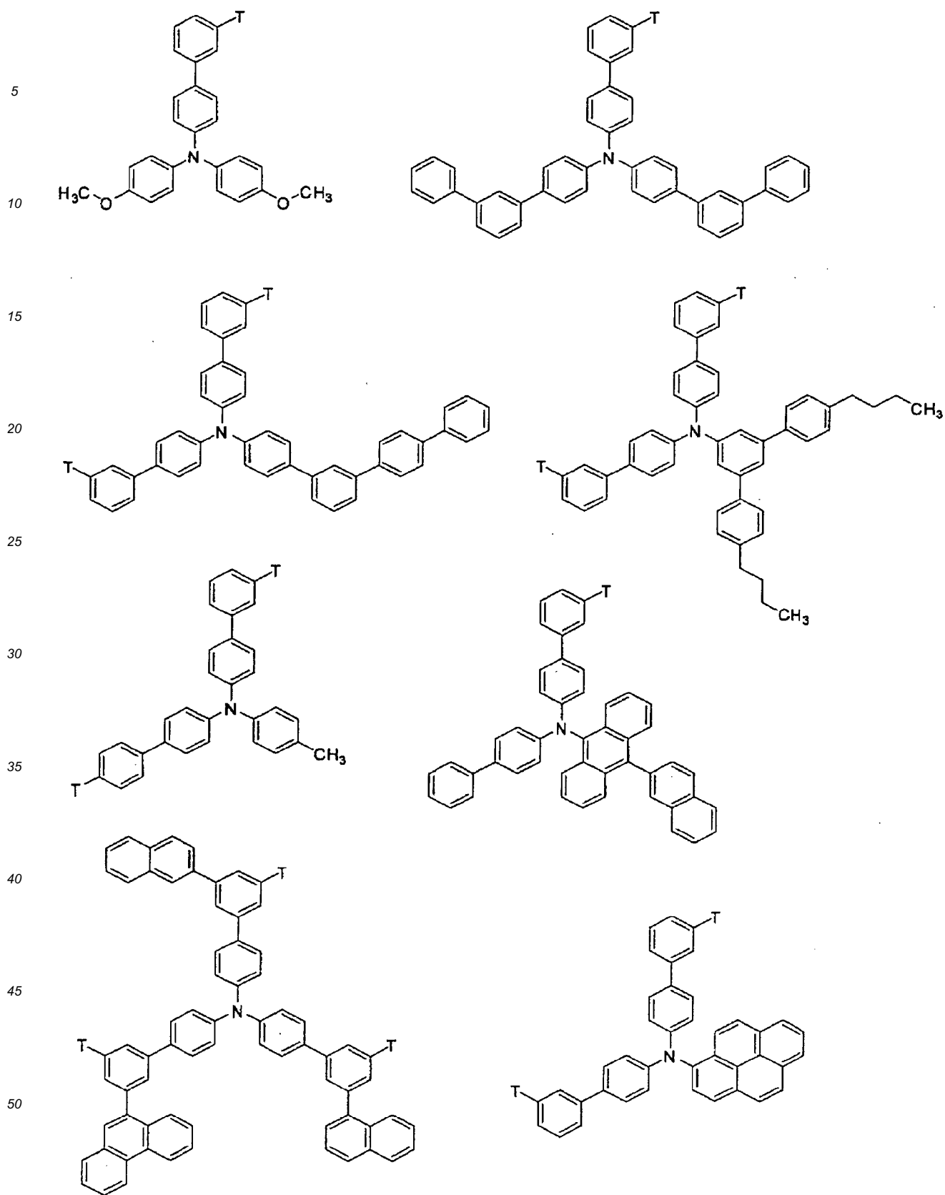
[Formula 12]
