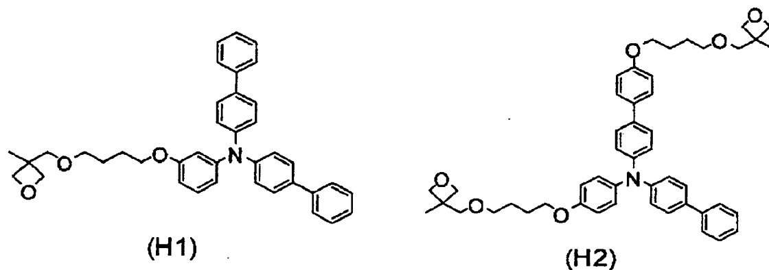
[Formula 99]
