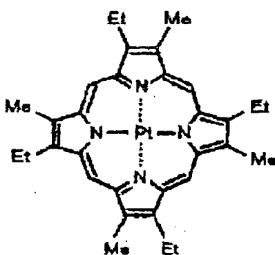
(D-2)
