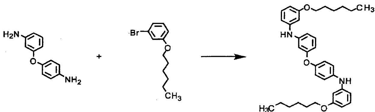
(Target compound 13)
