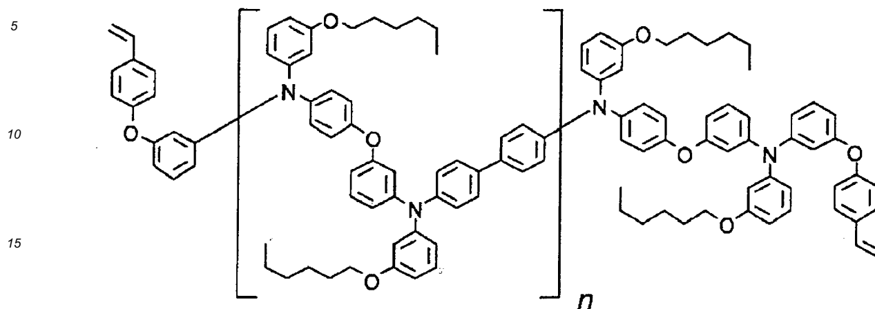
[Formula 33]
