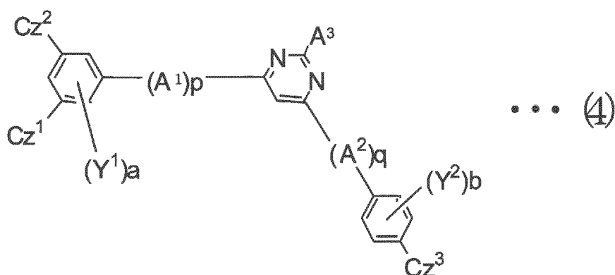
[Chemical Formula 8]
