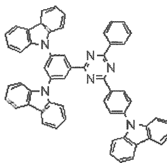
Compound No. 3
