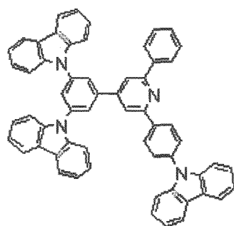
Compound No. 2
