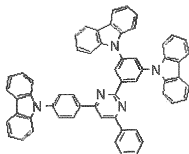
Compound No. 6
