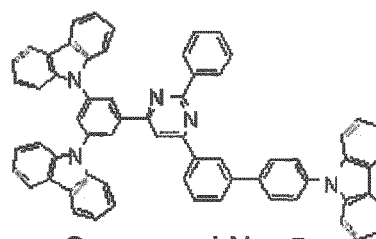
Compound No. 5
