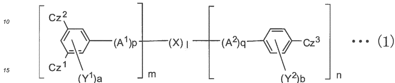
[Chemical Formula 5]
