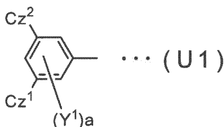
[Chemical Formula 2]
