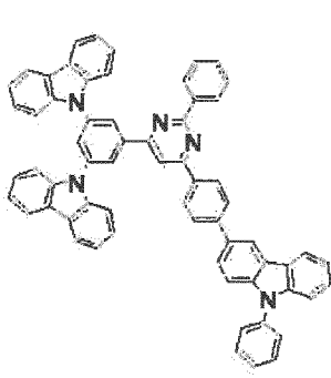
[Chemical Formula 26]
