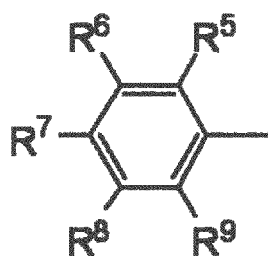
[Chemical Formula 57]
