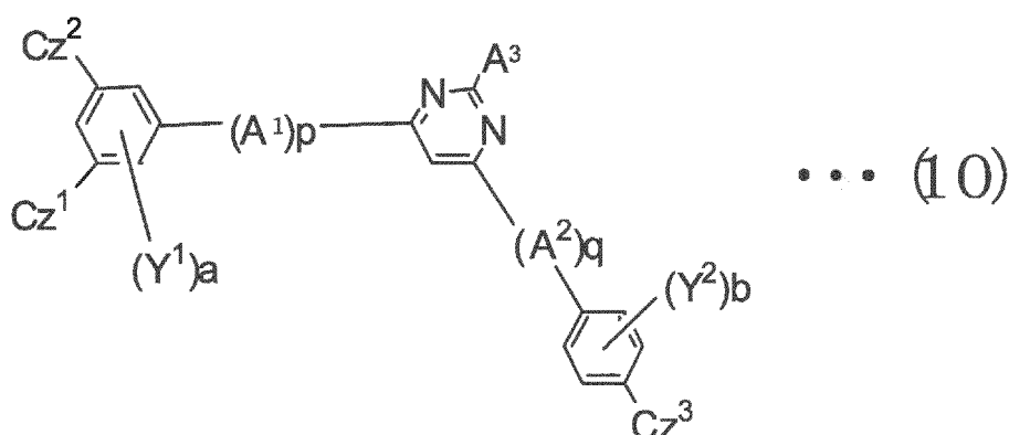
[Chemical Formula 19]
