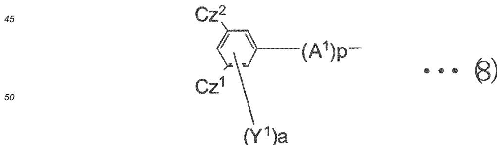
[Chemical Formula 15]
