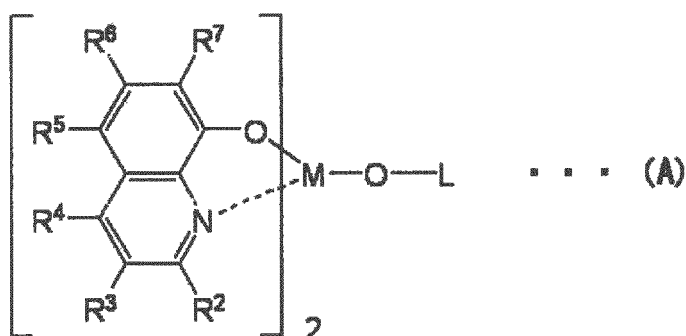
[Chemical Formula 44]
