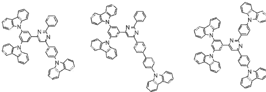
[Chemical Formula 25]
