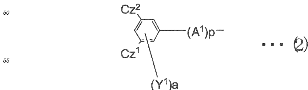
[Chemical Formula 6]
