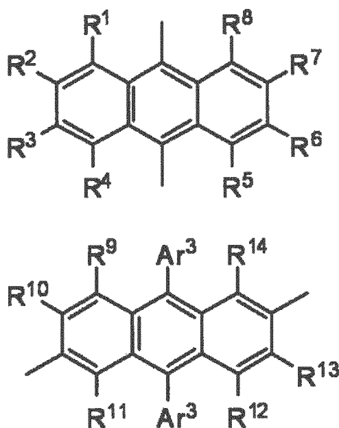
[Chemical Formula 53]
