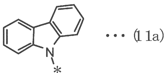
[Chemical Formula 23]
