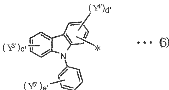
[Chemical Formula 6]
