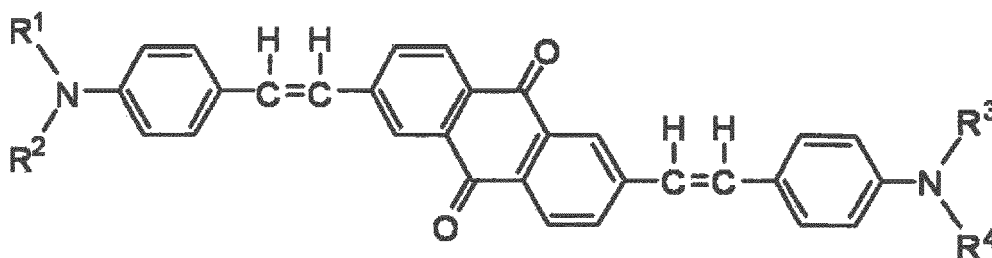
[Chemical Formula 56]
