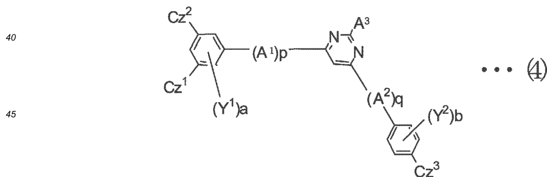
[Chemical Formula 4]
