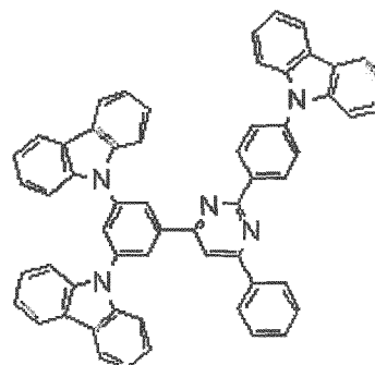
Compound No. 7
