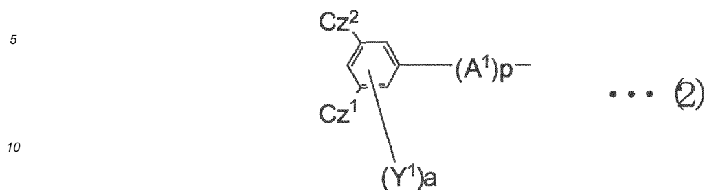
[Chemical Formula 2]
