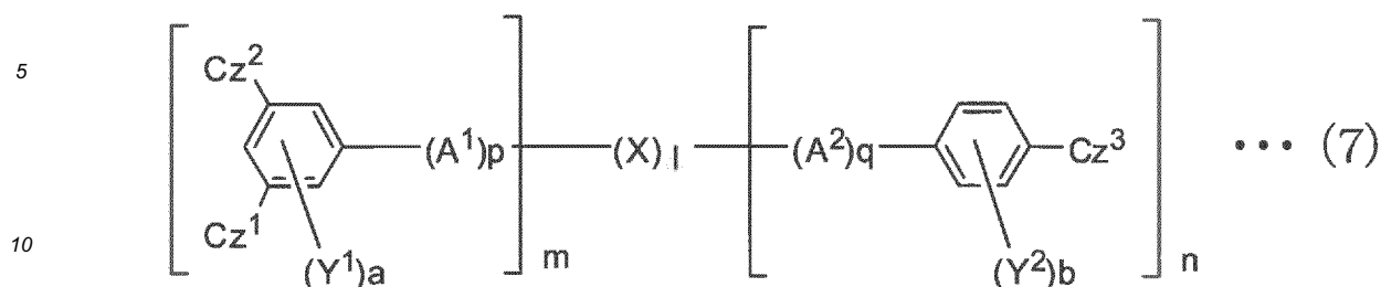
[Chemical Formula 14]
