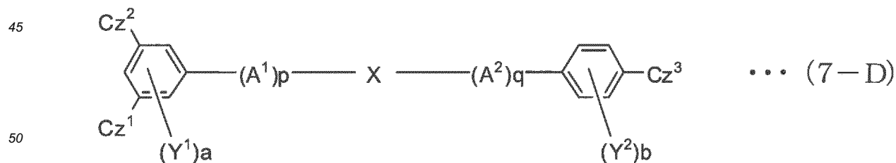
[Chemical Formula 18]
