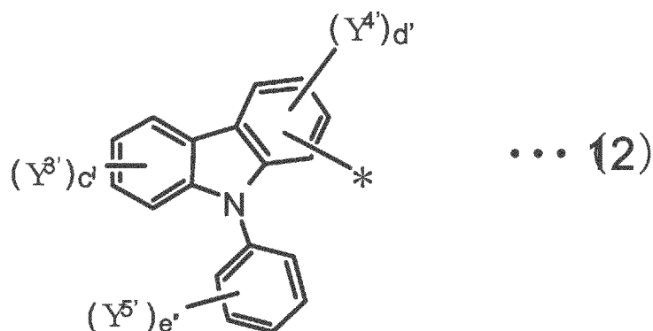
[Chemical Formula 22]
