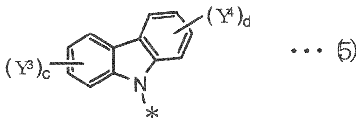
[Chemical Formula 5]
