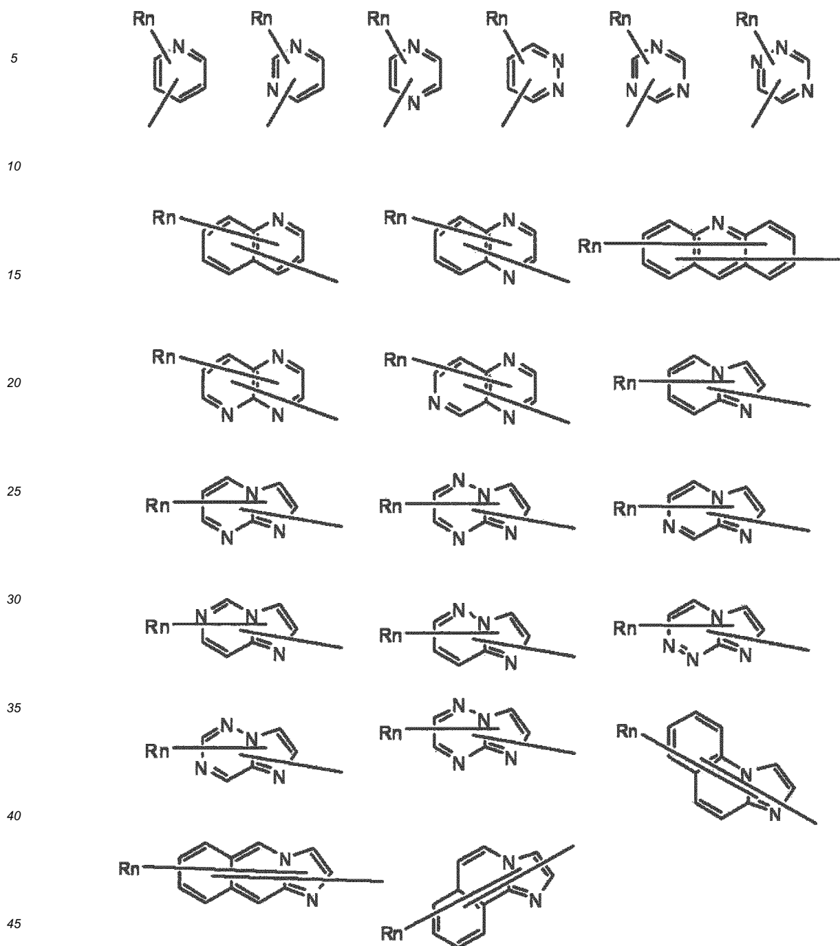
[Chemical Formula 50]
