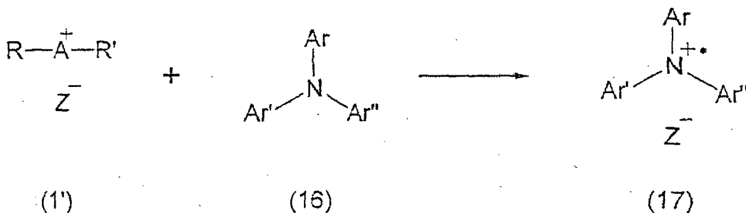
[Chemical Formula 24]
