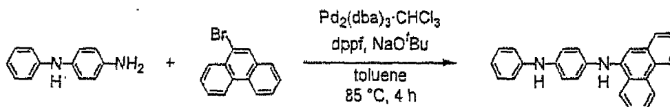
Compound 1
