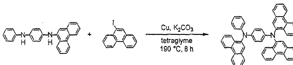
Compound 1
