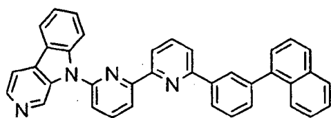
[Chem. 27]
