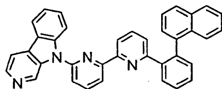
[Chem. 21]
