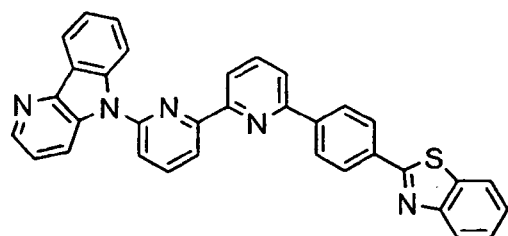
[Chem. 156]
