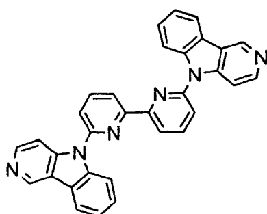
[Chem. 4]
