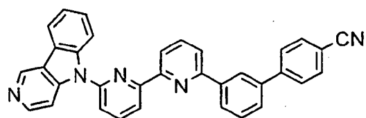
[Chem. 46]
