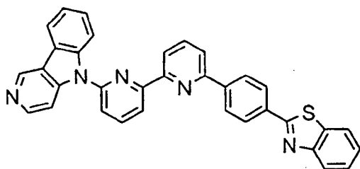
[Chem. 156]
