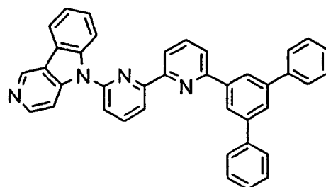
[Chem. 52]
