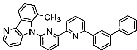
[Chem. 17]
