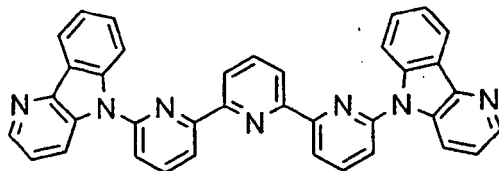
[Chem. 10]
