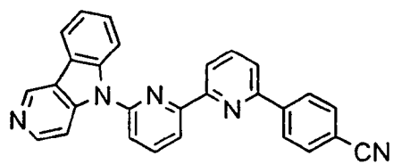
[Chem. 40]
