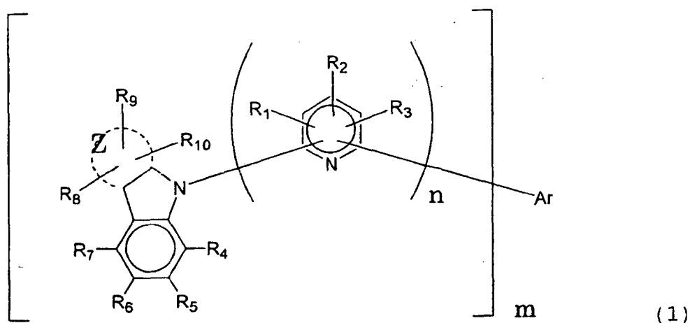
[Chem. 1]
