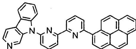
[Chem. 60]
