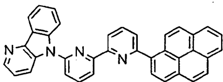
[Chem. 62]
