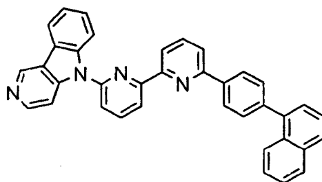
[Chem. 34]
