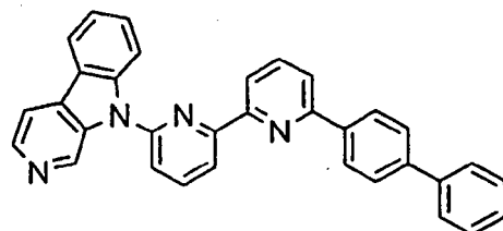
[Chem. 18]
