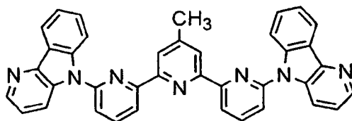
[Chem. 11]
