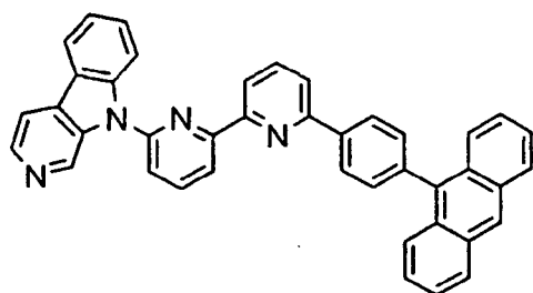
[Chem. 80]
