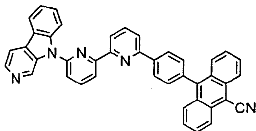
[Chem. 83]
