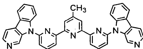
[Chem. 7]
