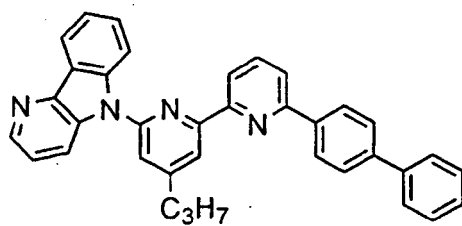
[Chem. 20]
