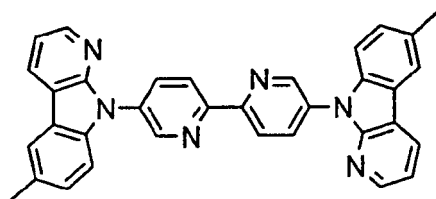
[Chem. 218]
