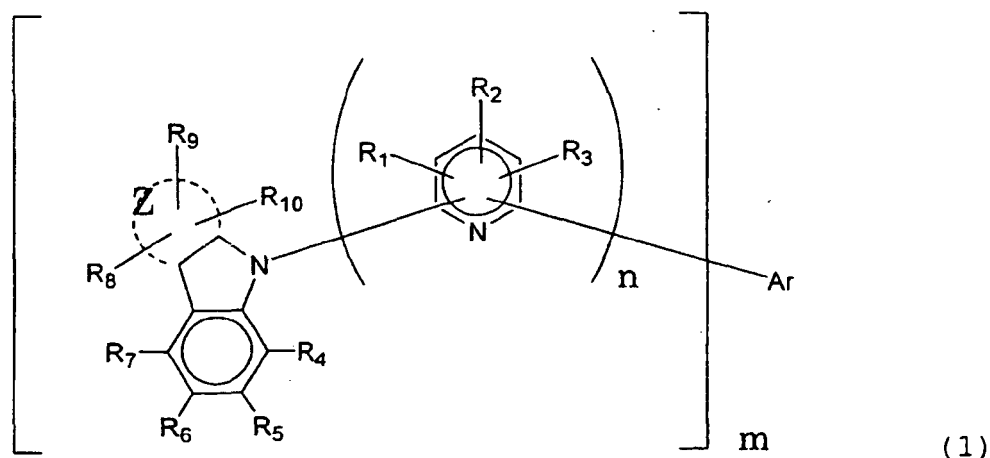
[Chem. 1]
