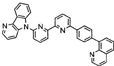
[Chem. 153]
