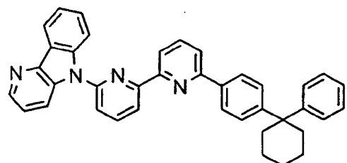
[Chem. 91]
