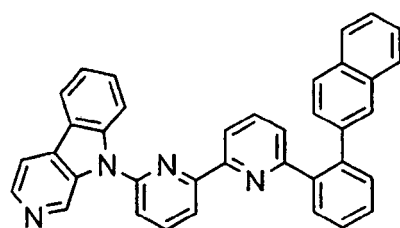
[Chem. 24]
