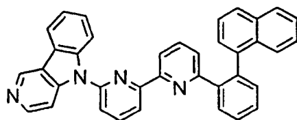
[Chem. 22]
