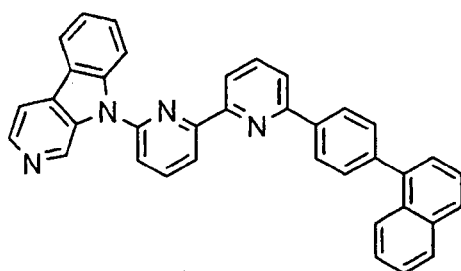
[Chem. 34]
