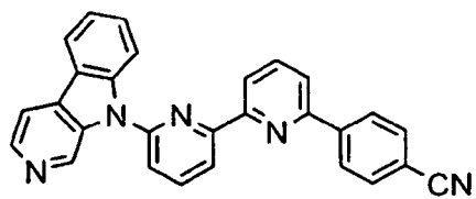
[Chem. 39]
