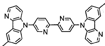
[Chem. 221]
