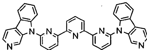
[Chem. 8]
