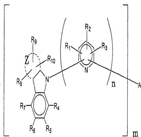
[Chem. 1]
