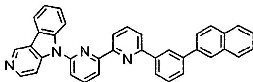
[Chem. 31]
