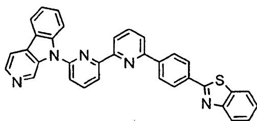
[Chem. 154]
