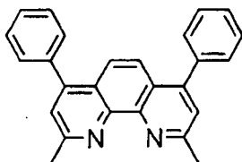
(Illustrative compound 1)
