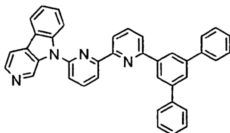
[Chem. 51]
