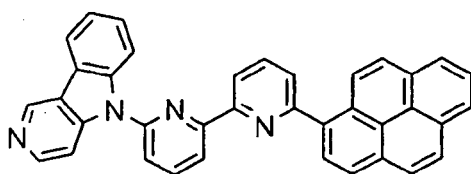
[Chem. 62]
