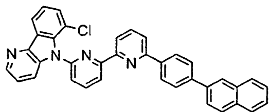
[Chem. 38]
