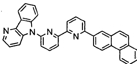
[Chem. 59]
