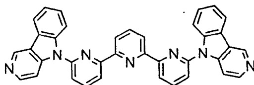
[Chem. 9]
