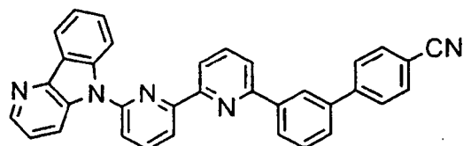
[Chem. 47]
