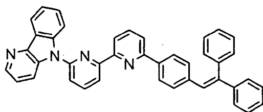
[Chem. 88]
