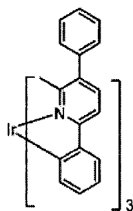
Compound 23
