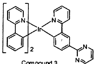
Compound 3
