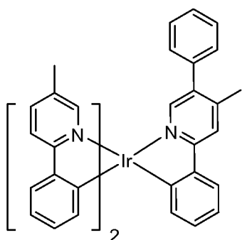
Compound 31
