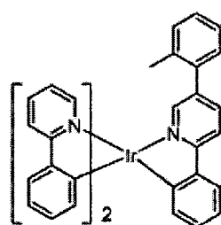
Compound 25
