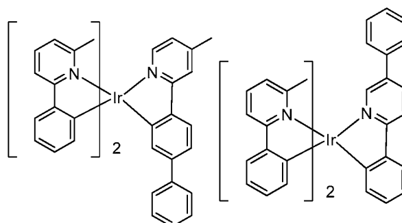
Compound 10
