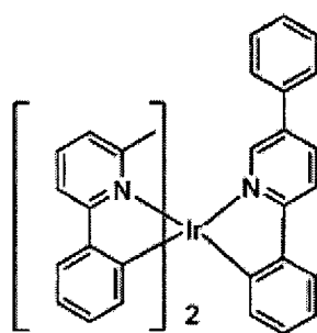
Compound 11
