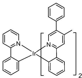
Compound 29
