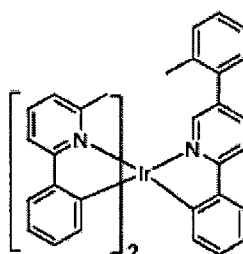
Compound 26
