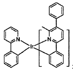
Compound 33
