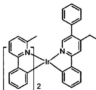
Compound 37
