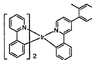
Compound 27
