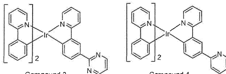
Compound 3
