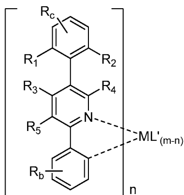
Formula V
