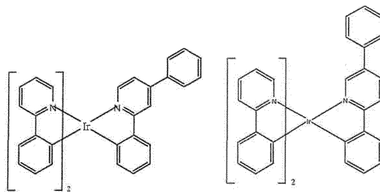
Compound 1
