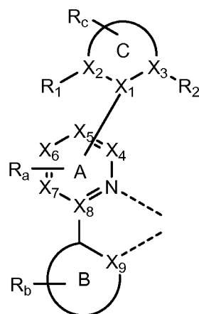
Formula I.
