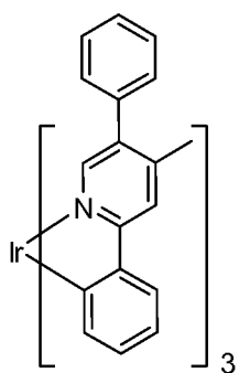
Compound 21
