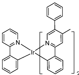
Compound 29
