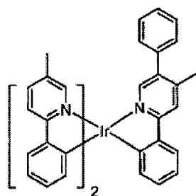
Compound 31
