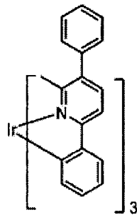
Compound 23
