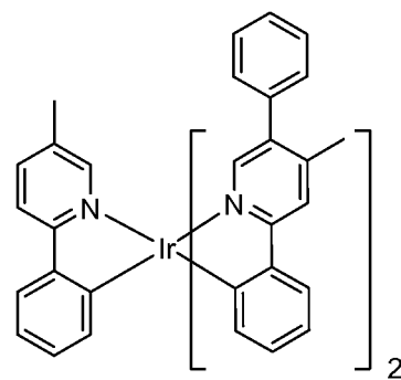
Compound 34
