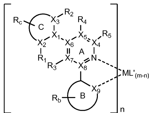
Formula IV
