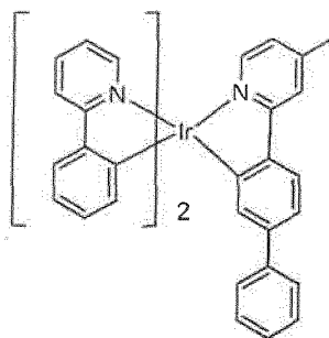
Compound 9
