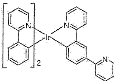
Compound 4
