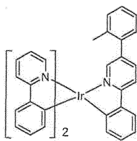
Compound 25
