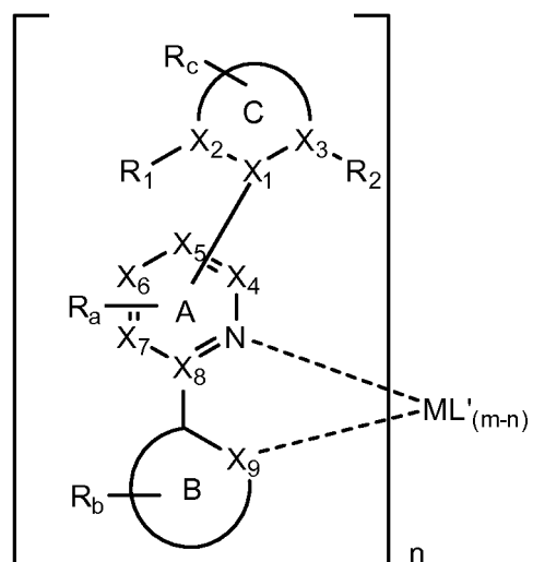
Formula II
