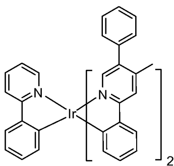
Compound 29
