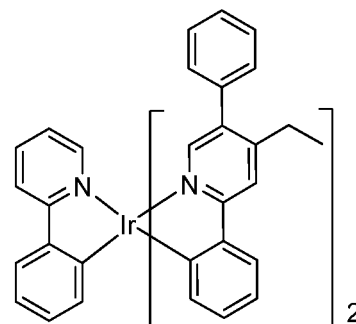
Compound 36
