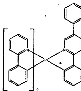
Compound 2
