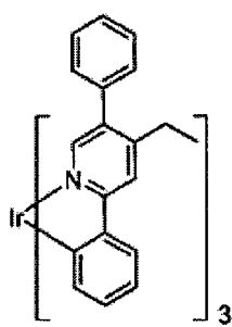
Compound 22
