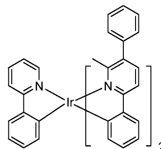
Compound 33
