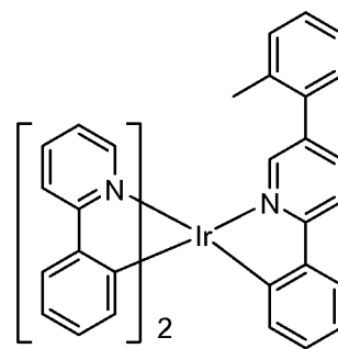
Compound 25
