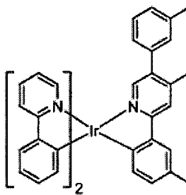
Compound 32
