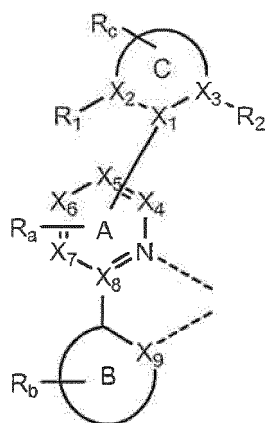
Formula I.
