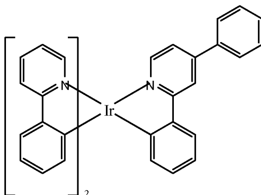
Compound 1
