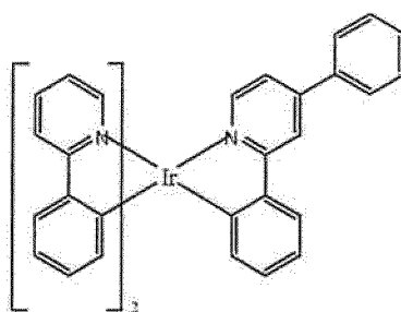
Compound 1
