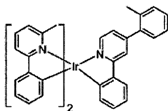
Compound 28
