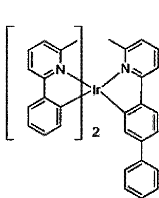
Compound 13
