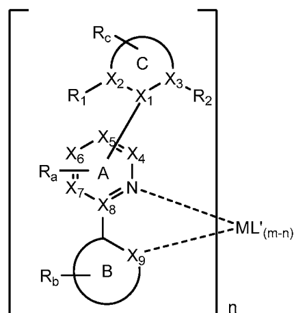
Formula II.
