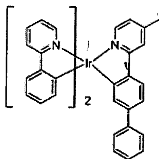
Compound 9
