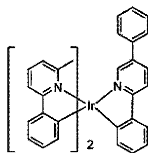
Compound 11
