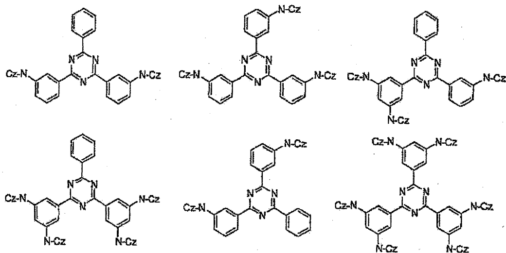
[Chem 16]
