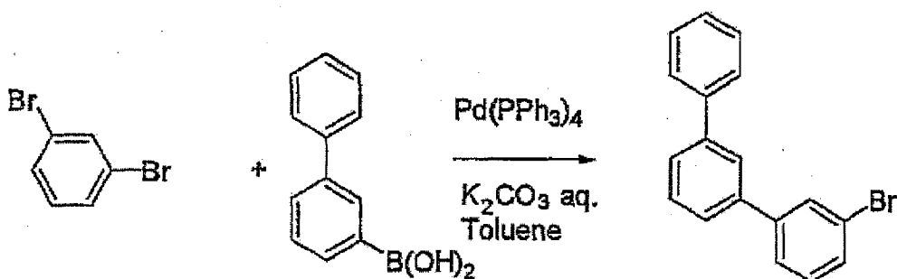
Objective compound 7
