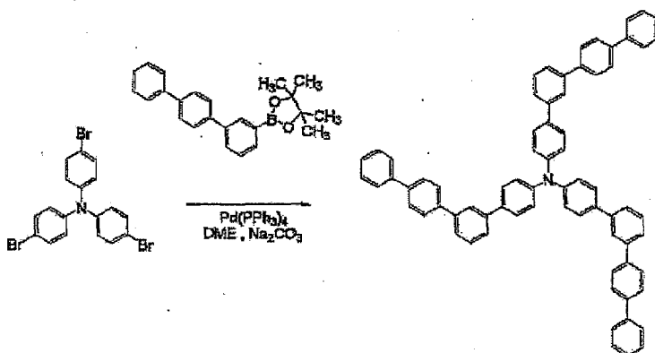
Objective compound 3
