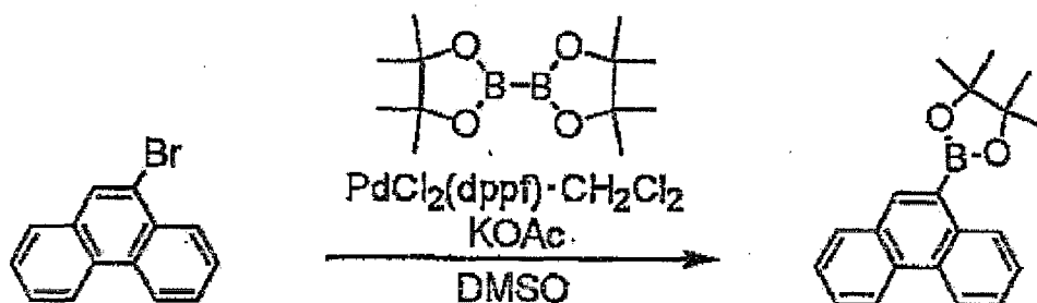
Objective compound 10
