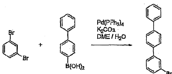
Objective compound 1
