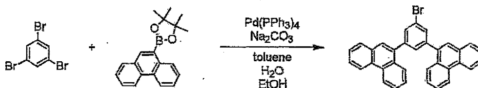
Objective compound 10
