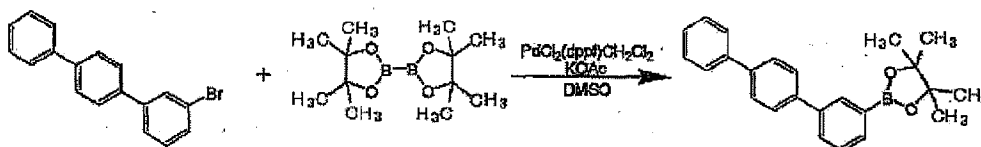
Objective compound 2
