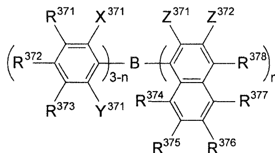
[Chemical Formula 22]
