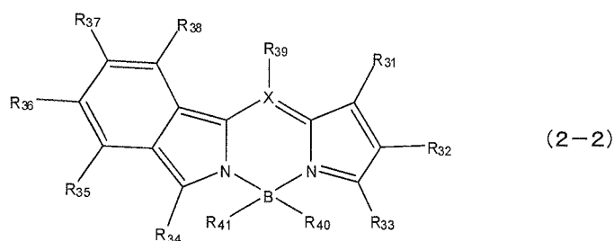
[Chemical Formula 4]
