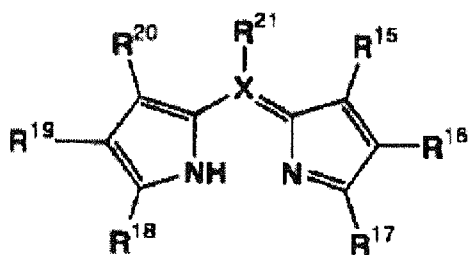
35 [Chemical Formula 2]
