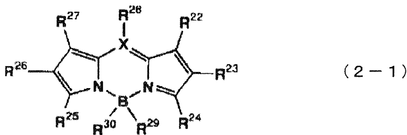
[Chemical Formula 3]
