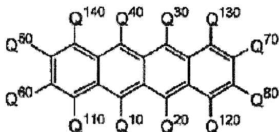
20 [Chemical Formula 1]
