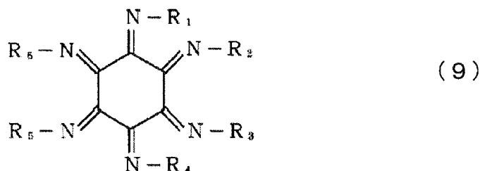
[Chemical Formula 16]
