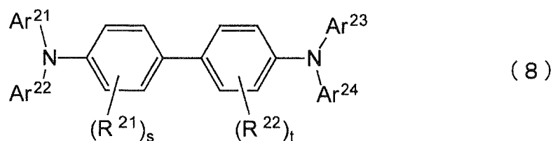
[Chemical Formula 15]
