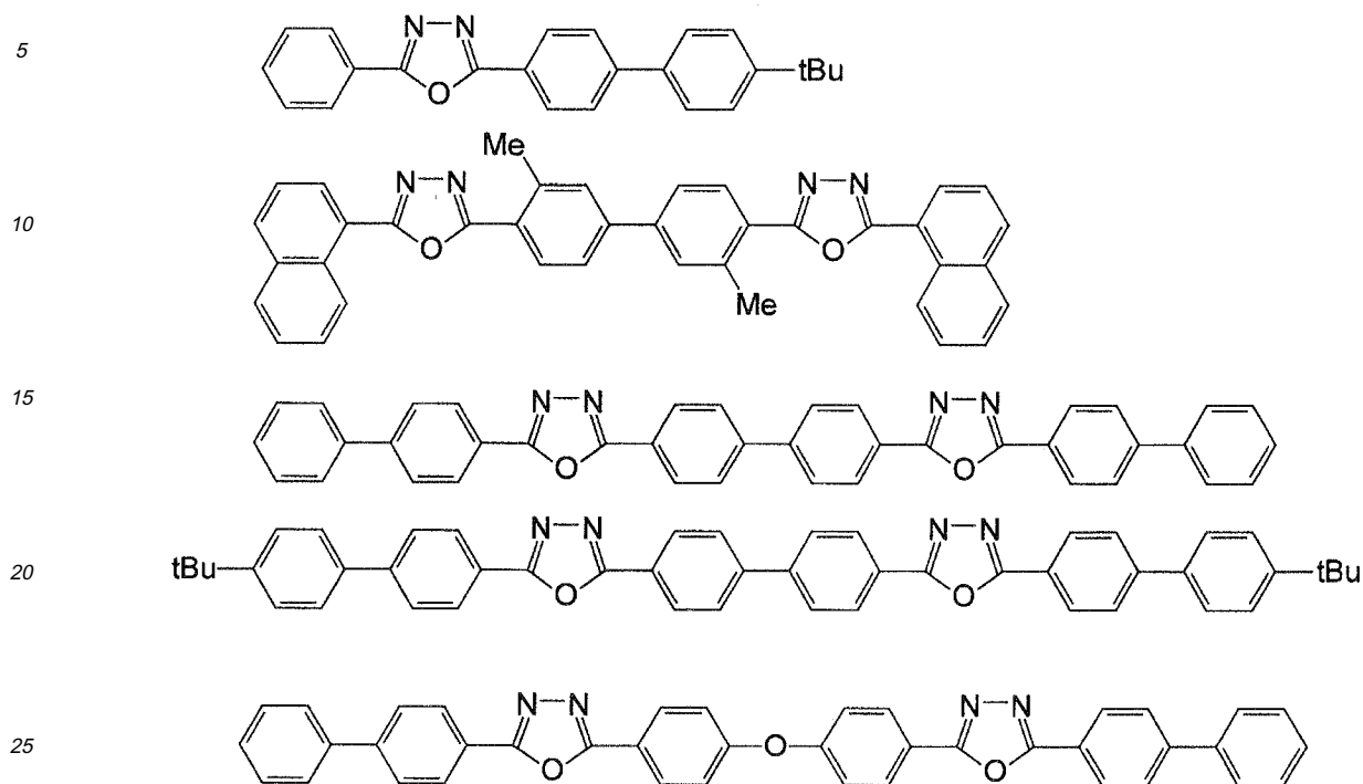
[Chemical Formula 19]
