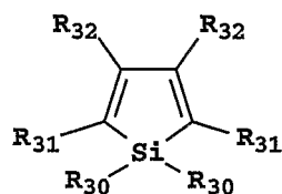
Formula IX
