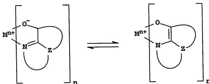
Formula I
