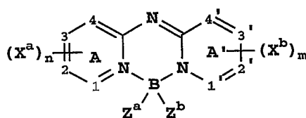
Formula III
