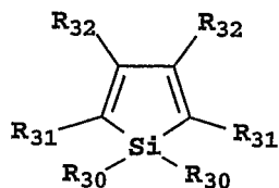
Formula IX
