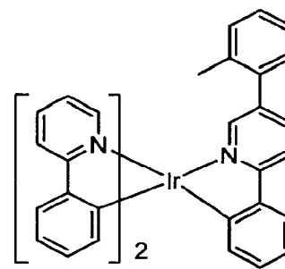
Compound 25
