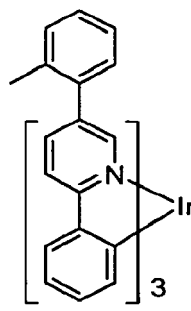
Compound 35
