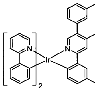
Compound 32
