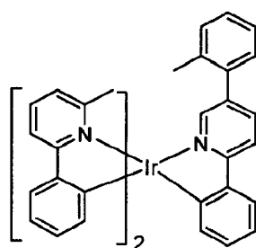
Compound 26
