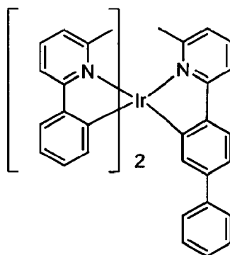
Compound 13
