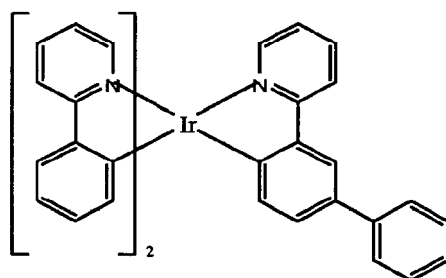
Compound 7
