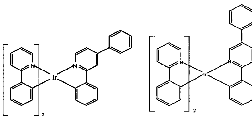
Compound 1
