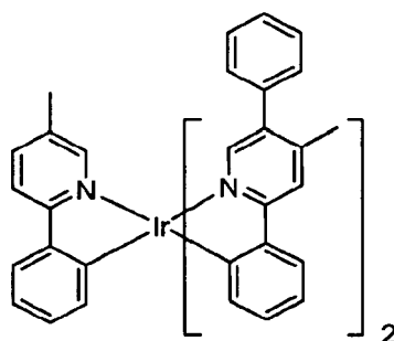
Compound 34
