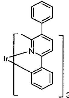
Compound 23
