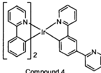
Compound 4
