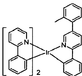
Compound 25
