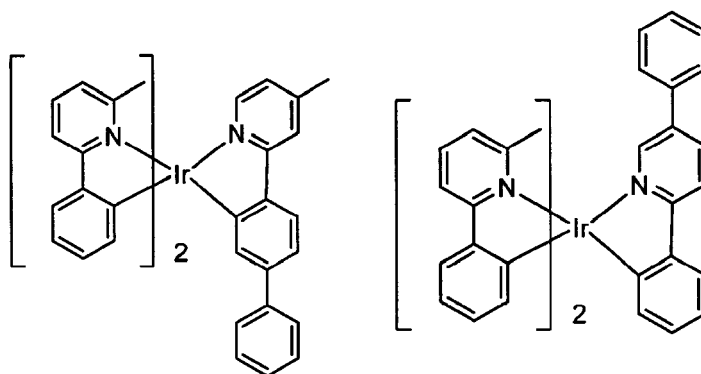
Compound 10
