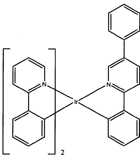
Compound 2
