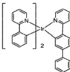
Compound 8
