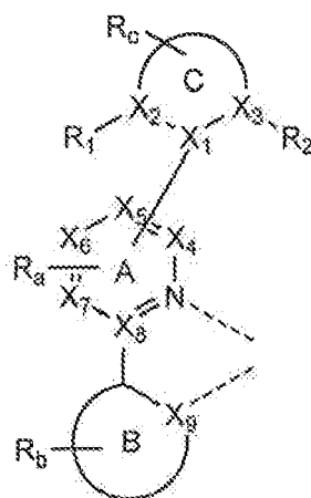
Formula I,
