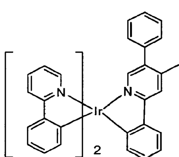
Compound 12
