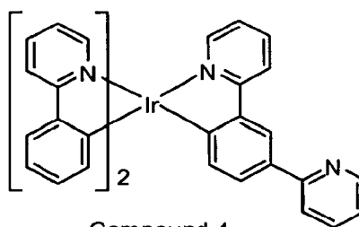
Compound 4
