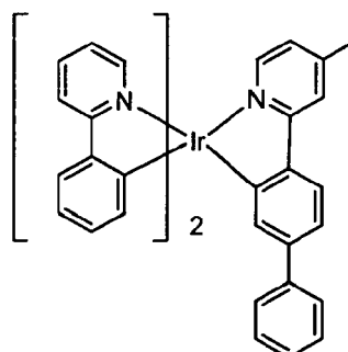
Compound 9
