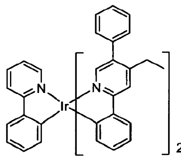
Compound 36
