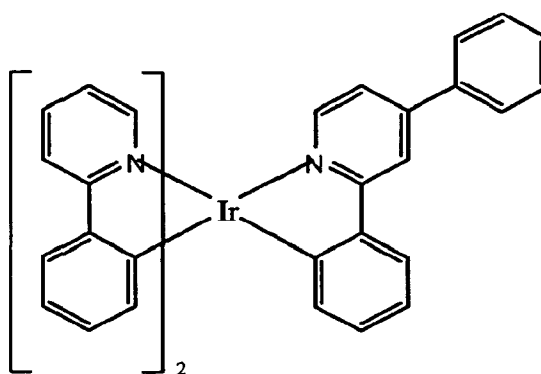
Compound 1
