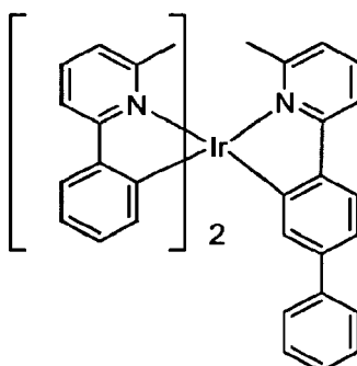
Compound 13
