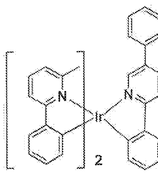
Compound 11
