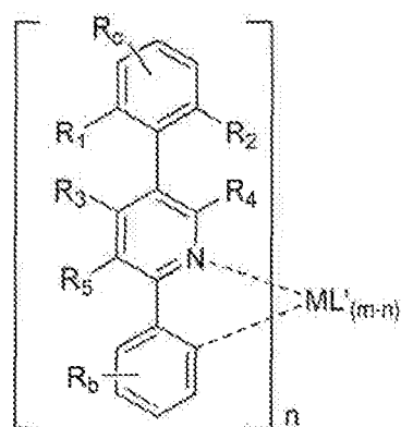
Formula V
