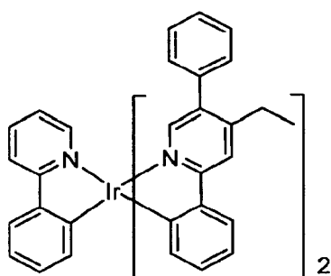
Compound 36
