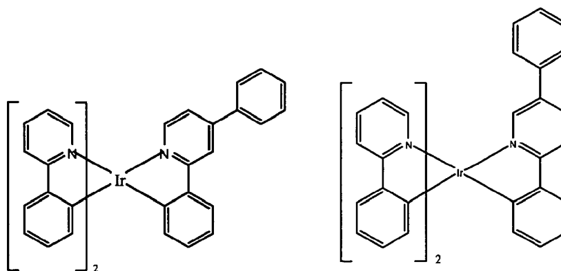
Compound 1
