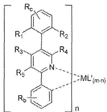
Formula V
