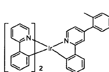
Compound 27
