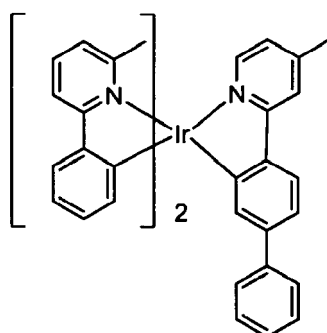
Compound 10
