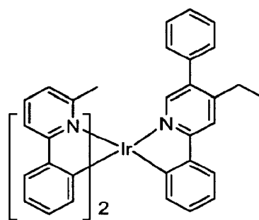
Compound 37
