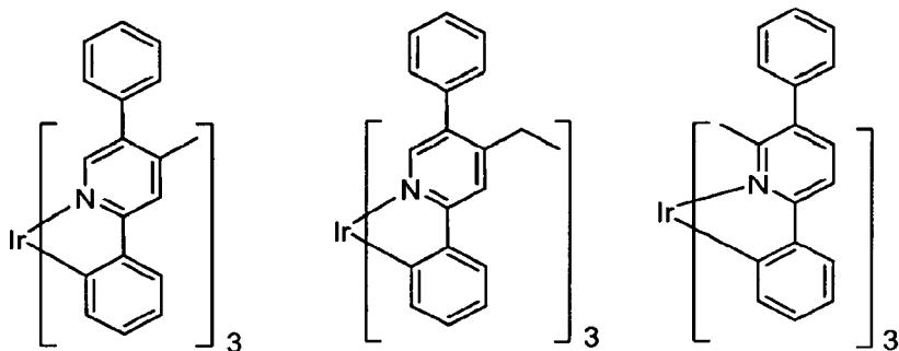
Compound 21
