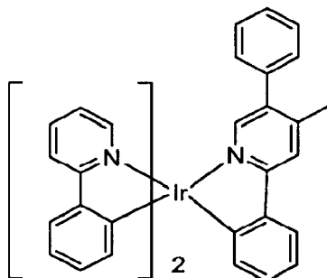
Compound 12
