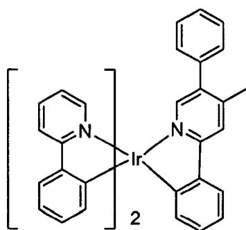
Compound 12
