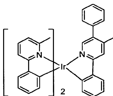
Compound 14
