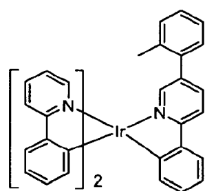
Compound 25
