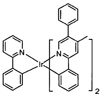
Compound 29
