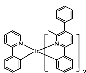
Compound 33
