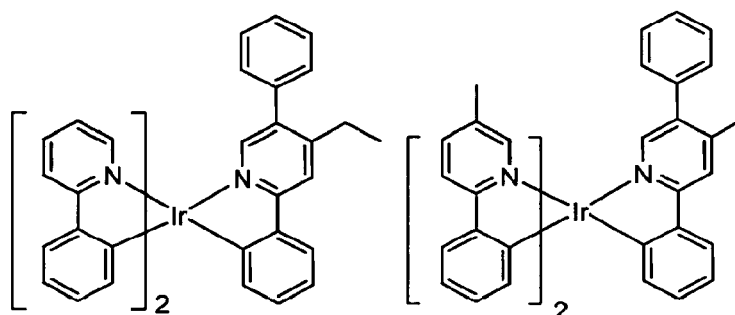
Compound 30
