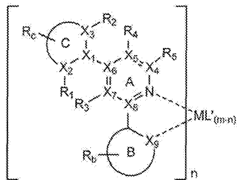
Formula IV
