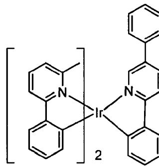
Compound 11
