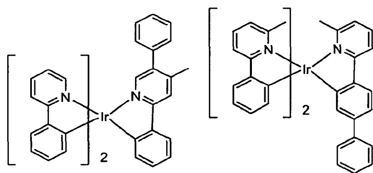
Compound 12
