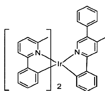
Compound 14
