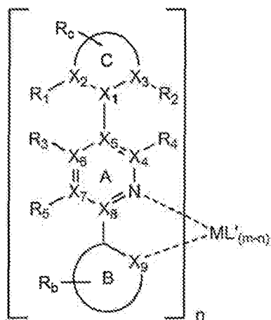
Formula III
