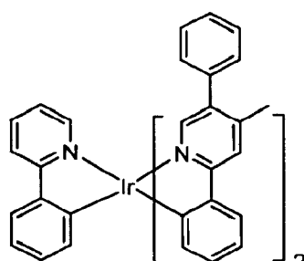
Compound 29
