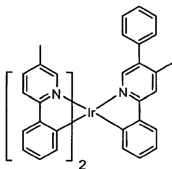
Compound 31
