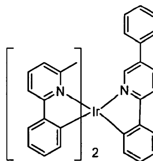
Compound 11
