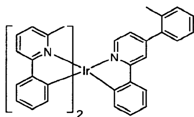
Compound 28
