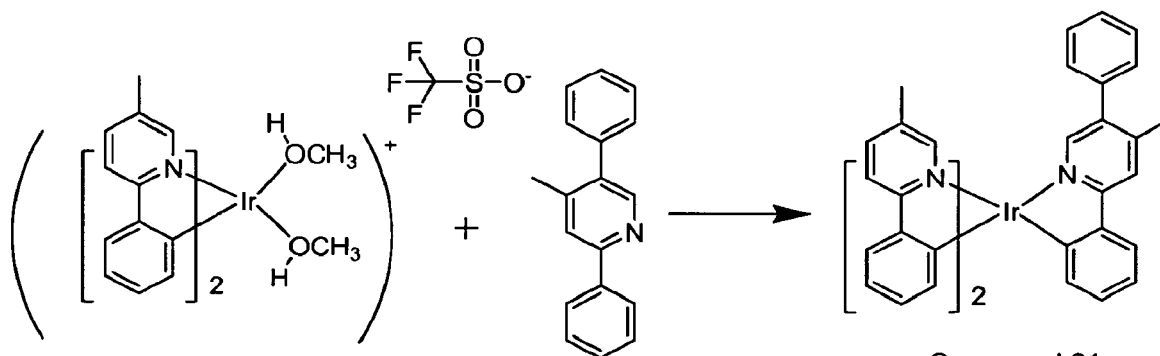
Compound 31
