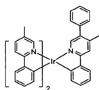
Compound 31
