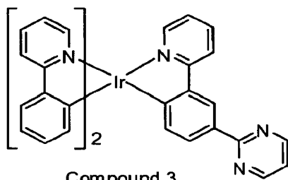
Compound 3
