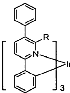
Compound 16
