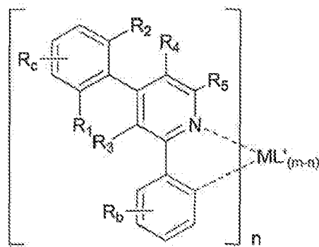
Formula VI
