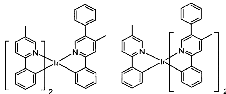
Compound 31
