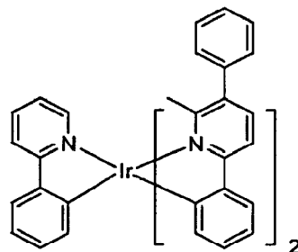
Compound 33
