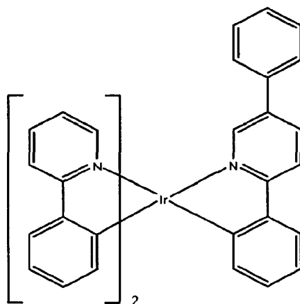
Compound 2
