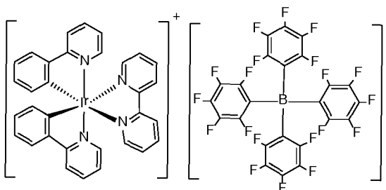
[Ir(ppy) 2 (bpy)][B(5fph) 4 ] formula (24)
