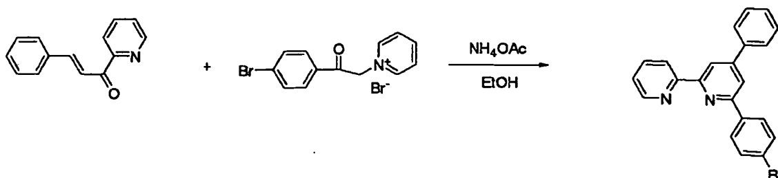
Target Compound 22
