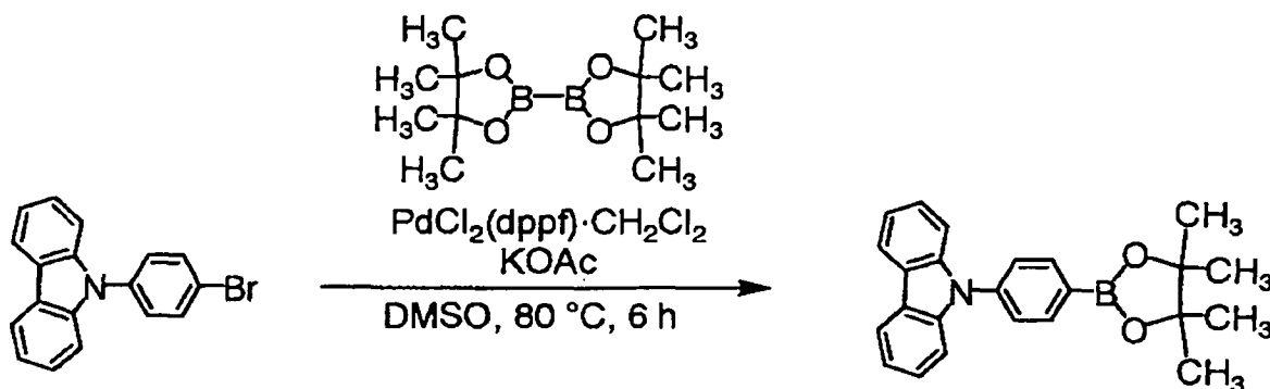
Target Compound 19
