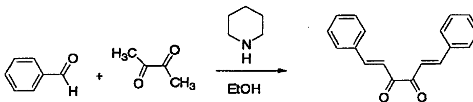
Target Compound 11
