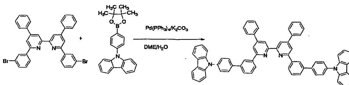
Target Compound 20
