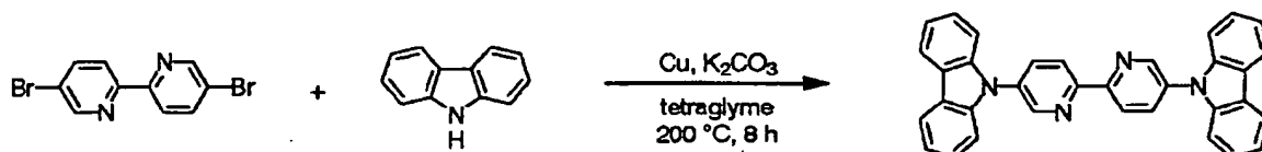
Target Compound 6
