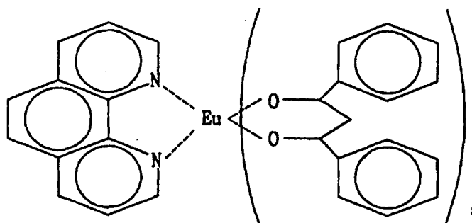
[Chemical Formula 2]
