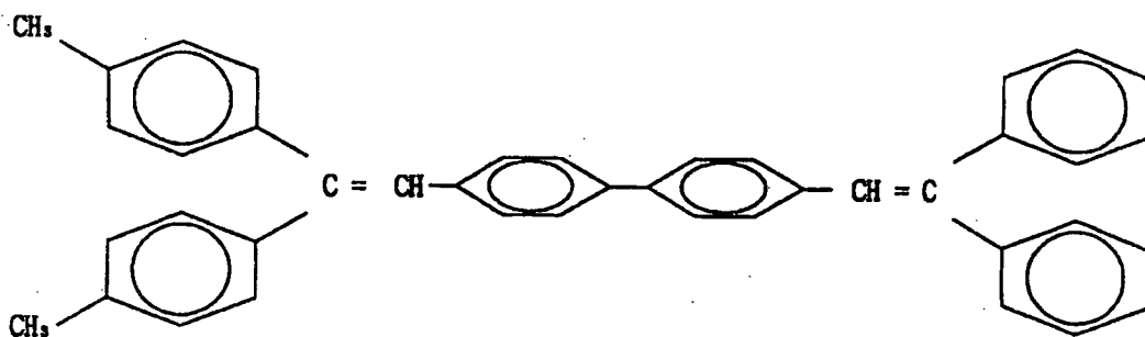
[Chemical Formula 3]
