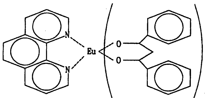
[Chemical Formula 2]
