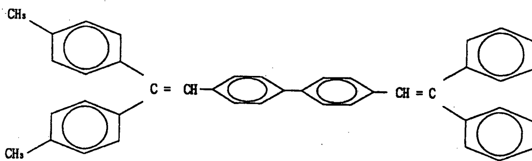
[Chemical Formula 3]
