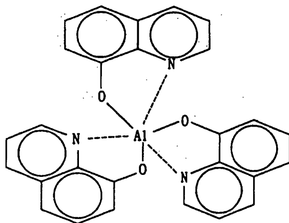
[Chemical Formula 2]
