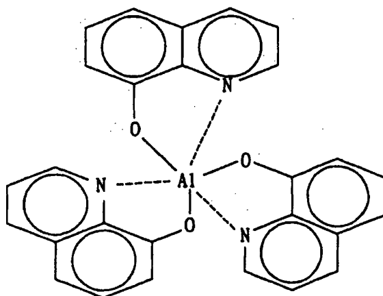
[Chemical Formula 2]
