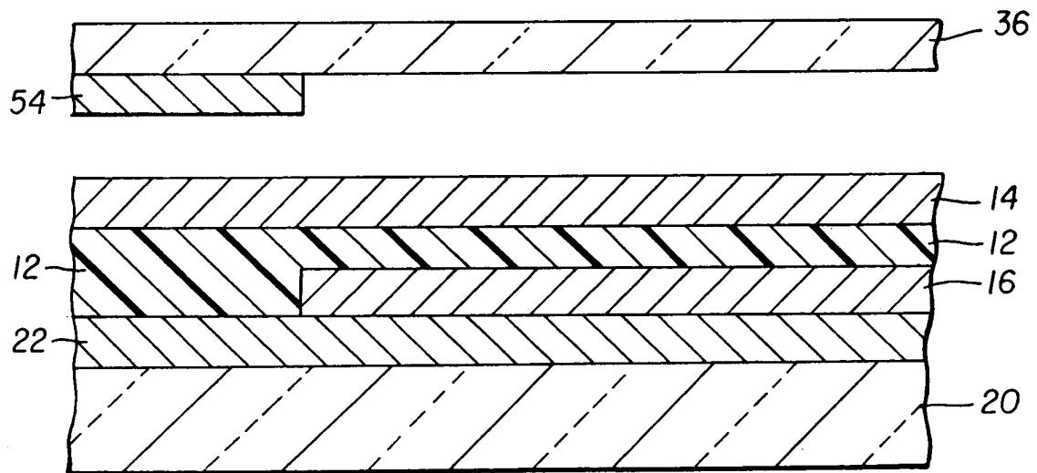
FIG. 2 (Prior Art)
