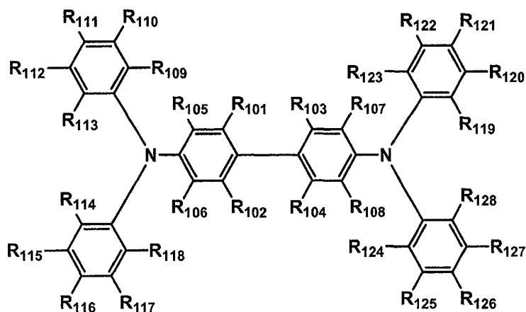
formula (IV)
