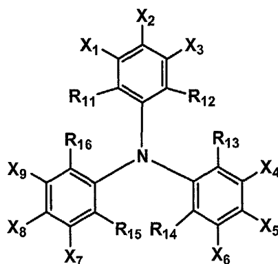
formula (III)
