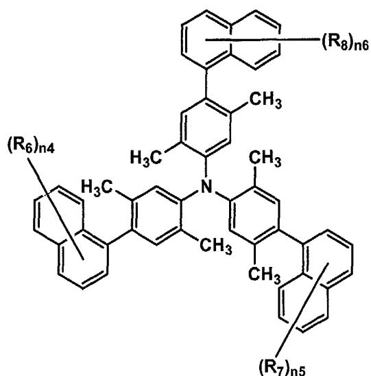
formula (II)
