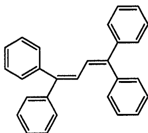
*TPB
