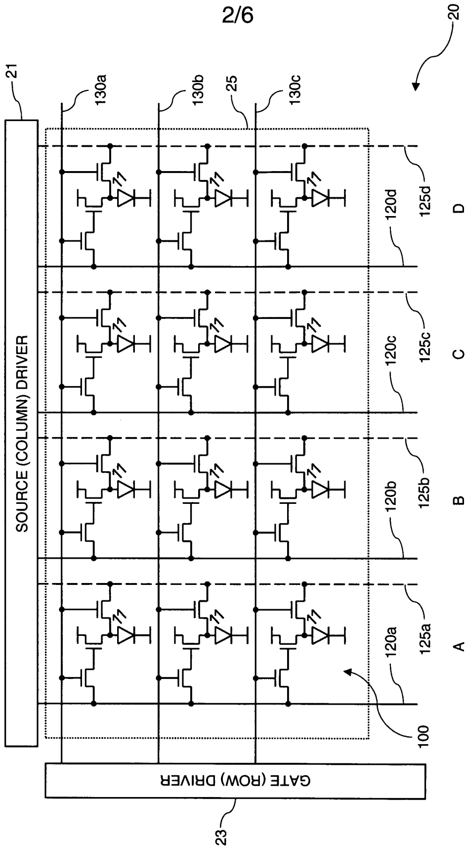
FIG. 2 (PRIOR ART)
