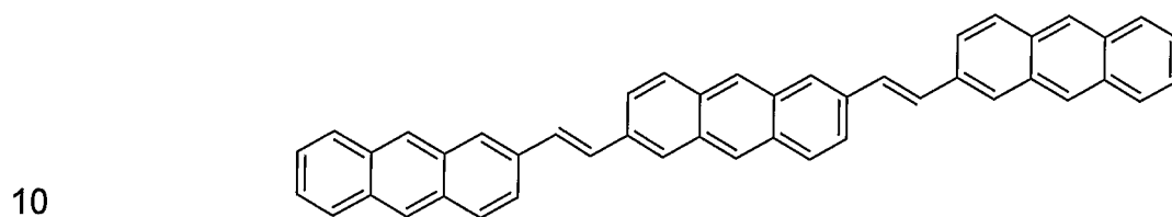
Compound 9
