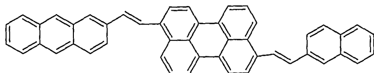
Compound 35
