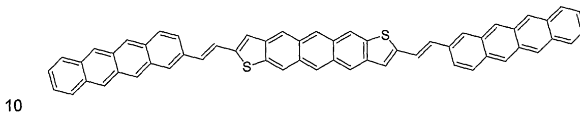
Compound 29
