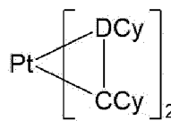
Formel (4)
