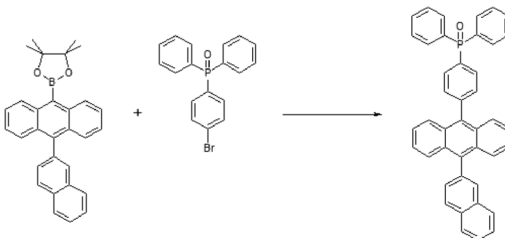
Structural Formula 1-4
