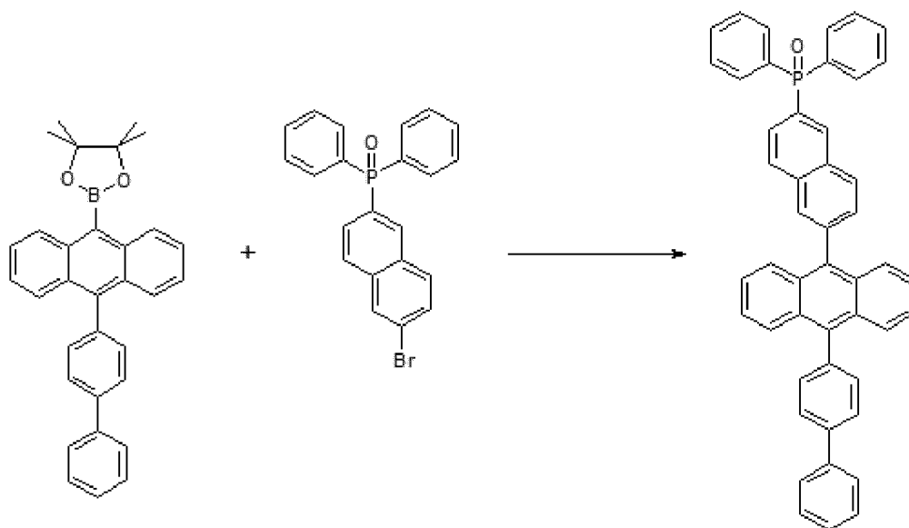
Structural Formula 1-9
