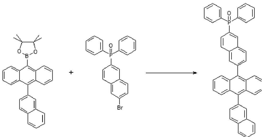
Structural Formula 1-8
