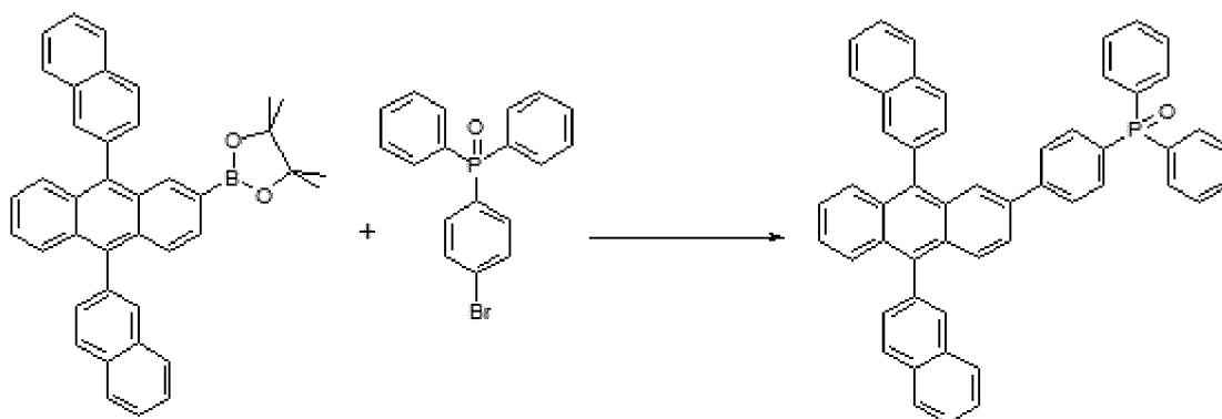
Structural Formula 1-3
