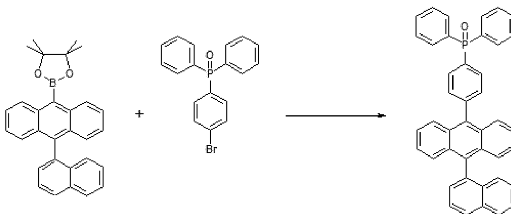
Structural Formula 1-2
