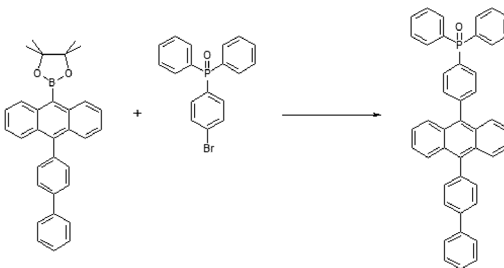
Structural Formula 1-5
