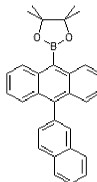
Structural Formula E
