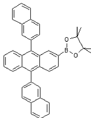
Structural Formula F
