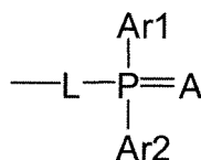
[Formula 2]
