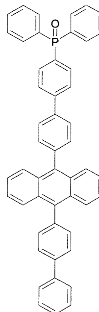
[Formula 1-6]
