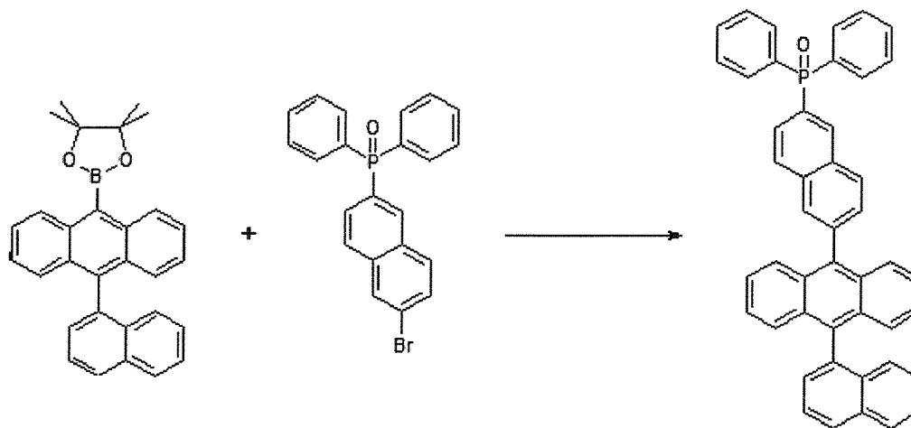
Structural Formula 1-7
