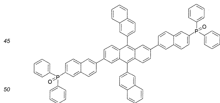
[Formula 1-22]
