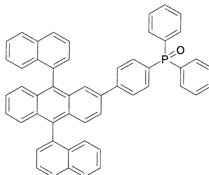
[Formula 1-15]
