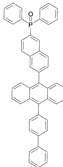
[Formula 1-9]
