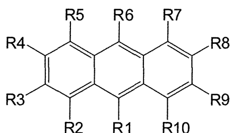
[Formula 1]
