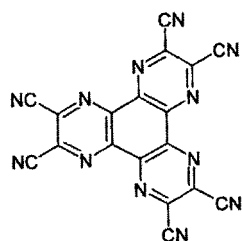
[hexanitrile hexaazatriphenylene]
