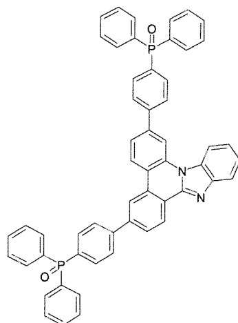
[Formula 1-45]
