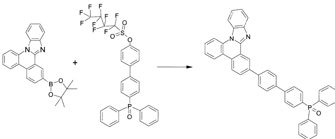
[Formula 1-7]
