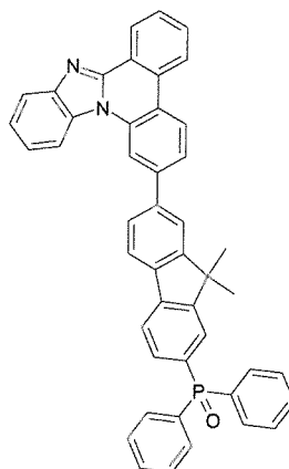
[Formula 1-39]
