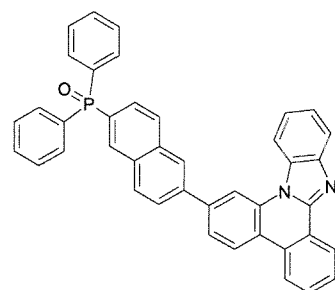
[Formula 1-13]
