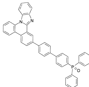
[Formula 1-7]
