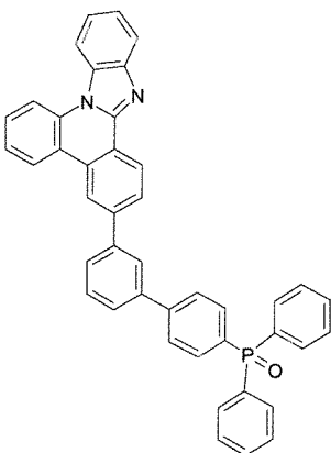
[Formula 1-21]
