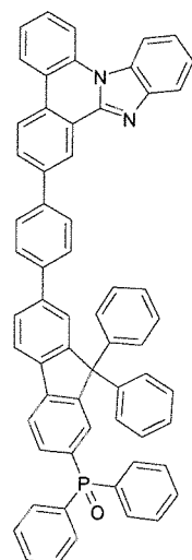
[Formula 1-29]
