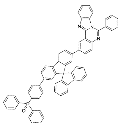
[Formula 1-25]
