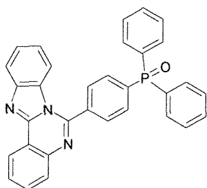
[Formula 1-4]
