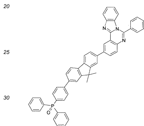
[Formula 1-24]
