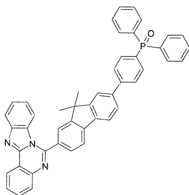
[Formula 1-16]
