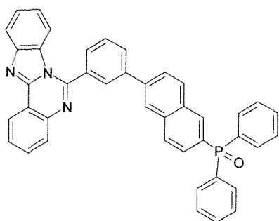
[Formula 1-7]
