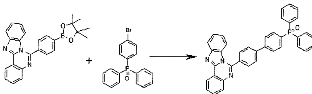
Structural Formula 1-2
