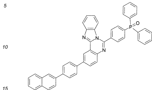
[Formula 1-21]
