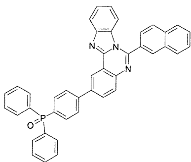
[Formula 1-10]
