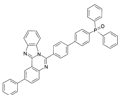
[Formula 1-13]
