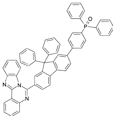
[Formula 1-17]
