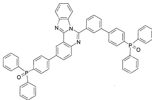
[Formula 1-26]
