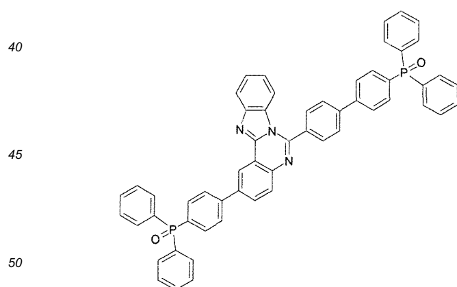
[Formula 1-24]
