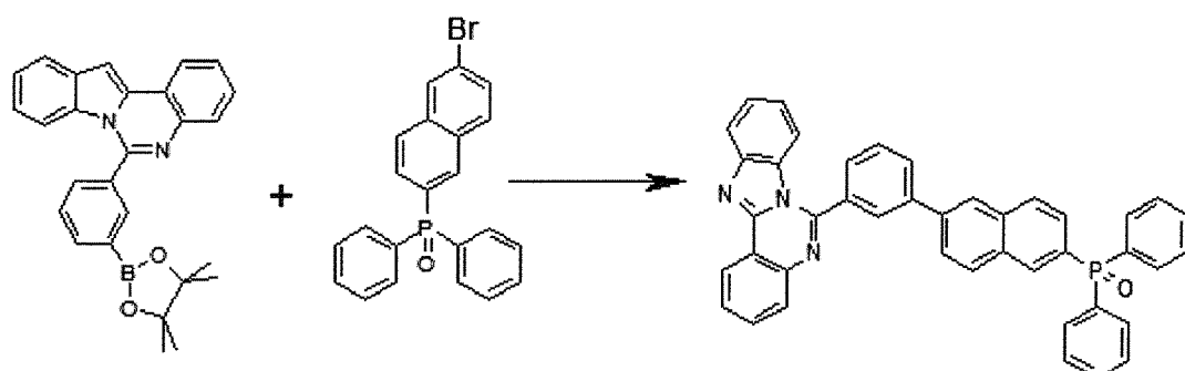
Structural Formula 1-4
