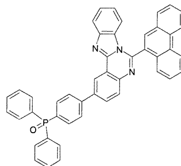
[Formula 1-12]
