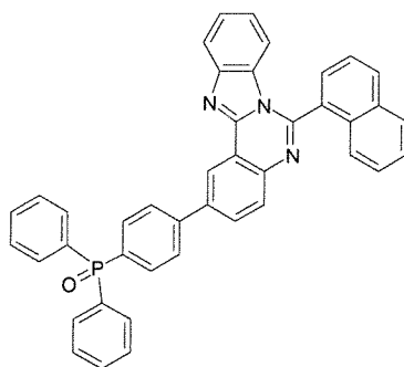
[Formula 1-11]
