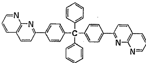
TPM-dNTR
