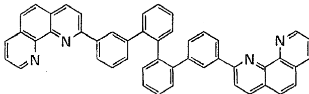
Phen-3
