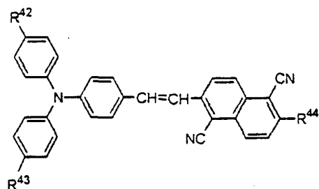
Formula (6)
