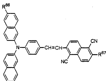
Formula (16)
