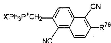
Formula (19)
