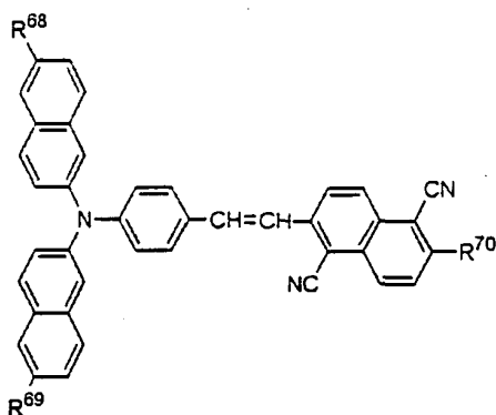
Formula (17)
