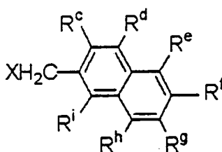
Formula [E]
