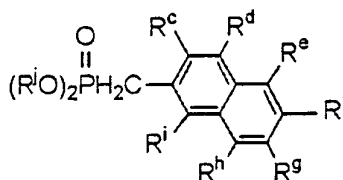
Formula [C]
