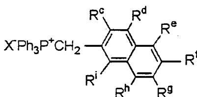
Formula [D]
