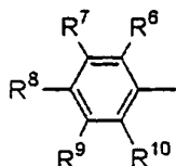
Formula (1)
