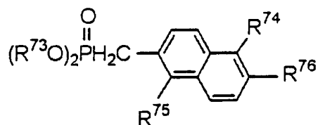
Formula [V]
