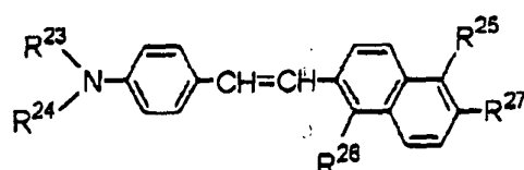
Formula [III]
