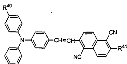
Formula (5)
