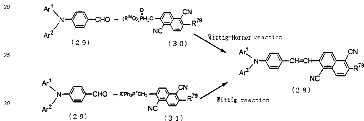
Reaction Scheme 1
