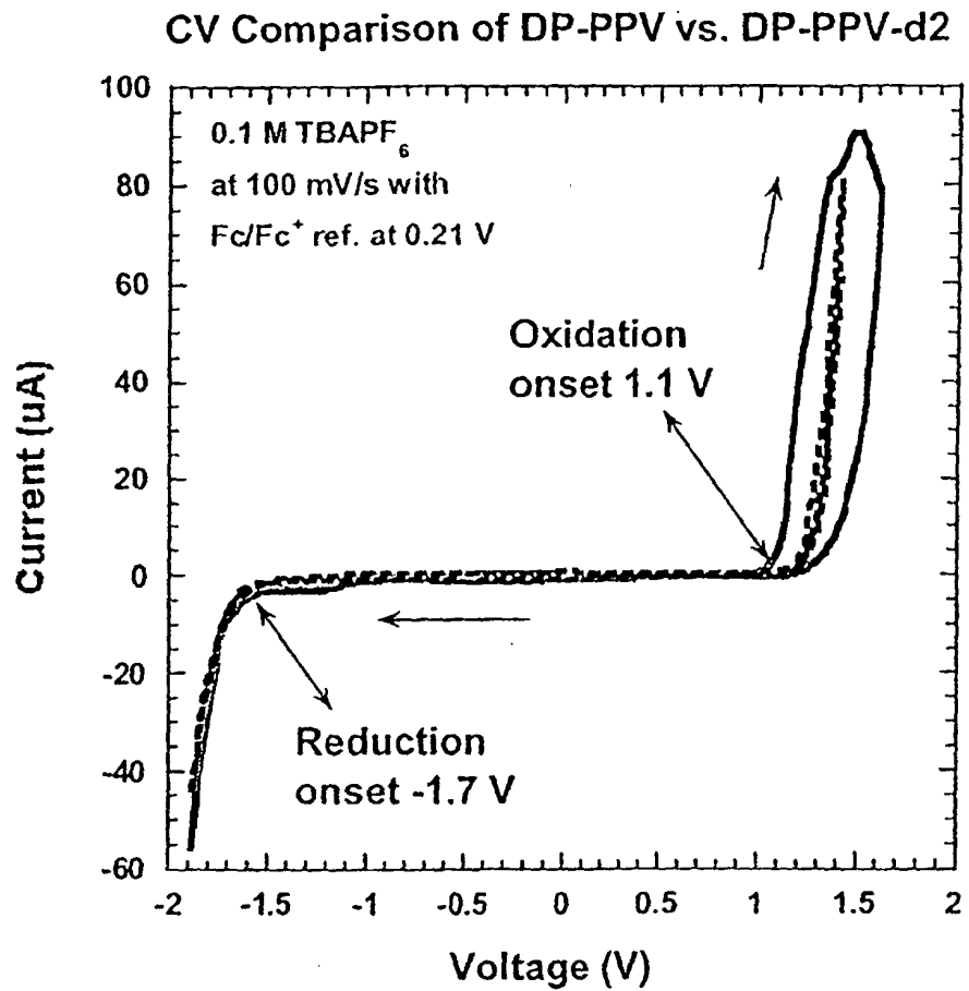
Figure 2. Cyclic voltammetric curve of normal DP-PPV (dotted line in blue) and d2-terminated DP-PPV-d2 (solid line).
