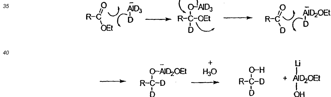
Scheme 2. Deuterium reaction mechanism
