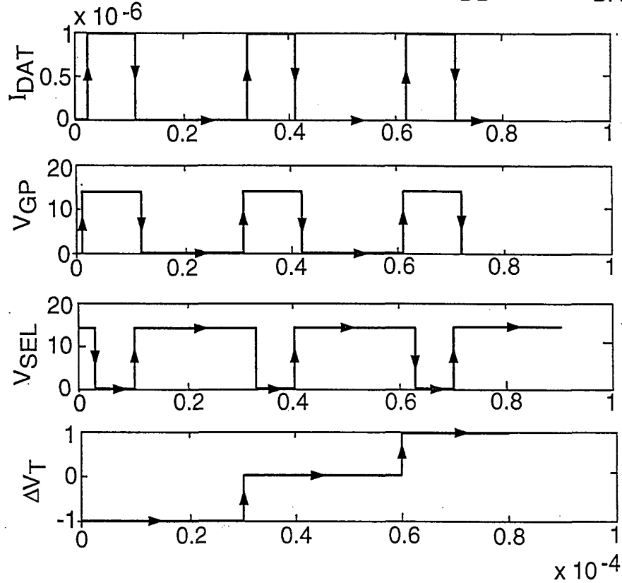
Fig.8. SPICE Simulation Result ( V_{DD}=12.5V , I_{DAT}=1\mu A )
