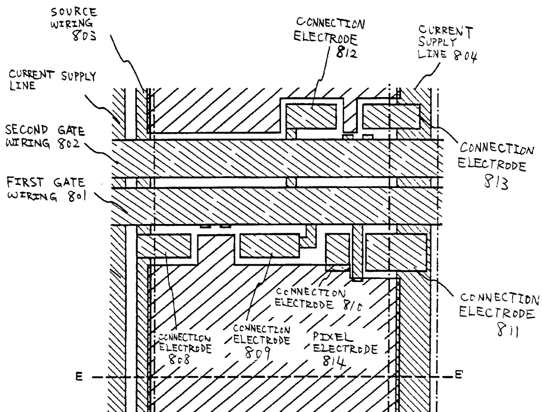
Fig. 10A TOP VIEW
