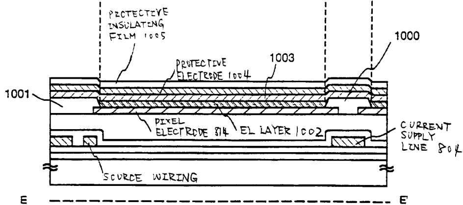
Fig. 10B E-E' CROSS-SECTIONAL VIEW
