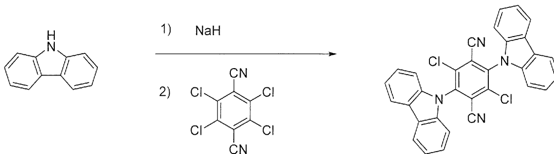
Intermediate 1
