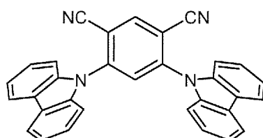
Comparative Compound 3-1
