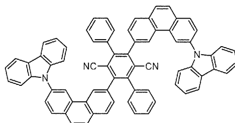
Invention Compound 9-3
