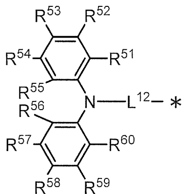
General Formula (4)
