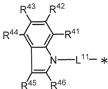
General Formula (3)
