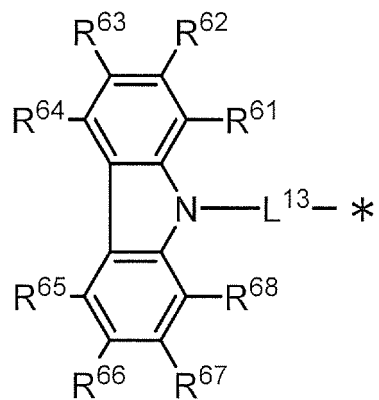
General Formula (5)
