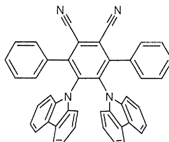
Invention Compound 1-1
