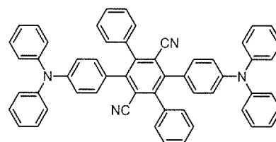
Invention Compound 10-1
