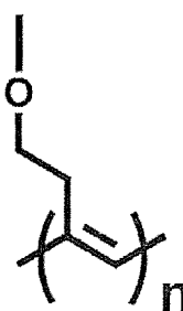
Formula (6)
