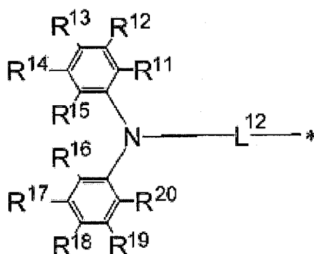
General Formula (3)
