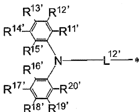
General Formula (2')
