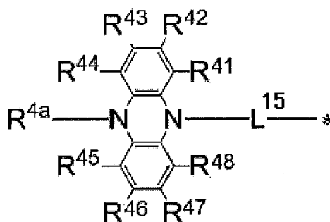
General Formula (6)
