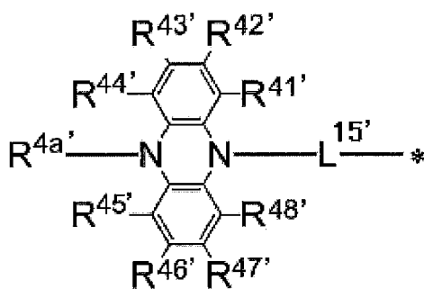
General Formula (5')
