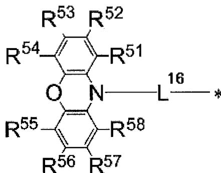
General Formula (7)
