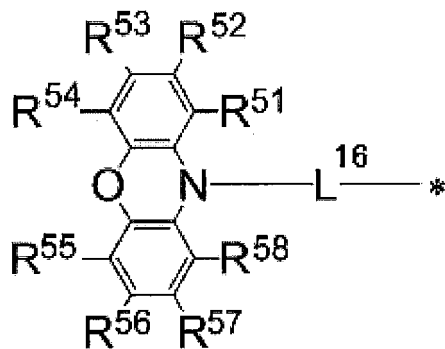
General Formula (6)
