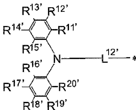
General Formula (3')
