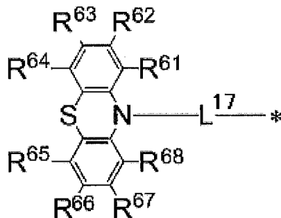
General Formula (7)
