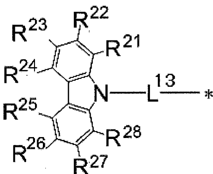
General Formula (4)
