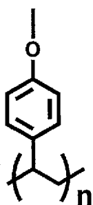
Formula (13)
