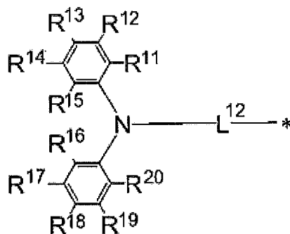
General Formula (3)
