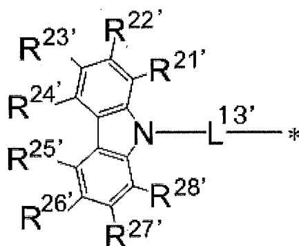
General Formula (4')
