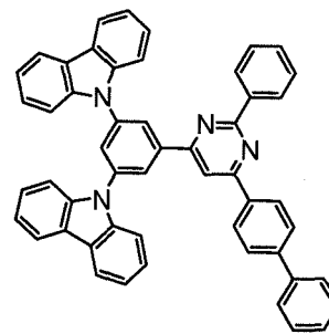
Compound F3
