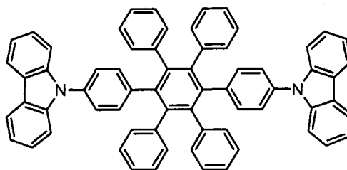
[Chemical Formula 24]
