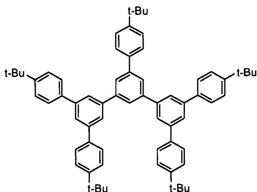
[Chemical Formula 19]
