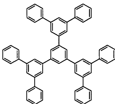
[Chemical Formula 18]
