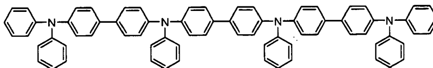
[Chemical Formula 11]
