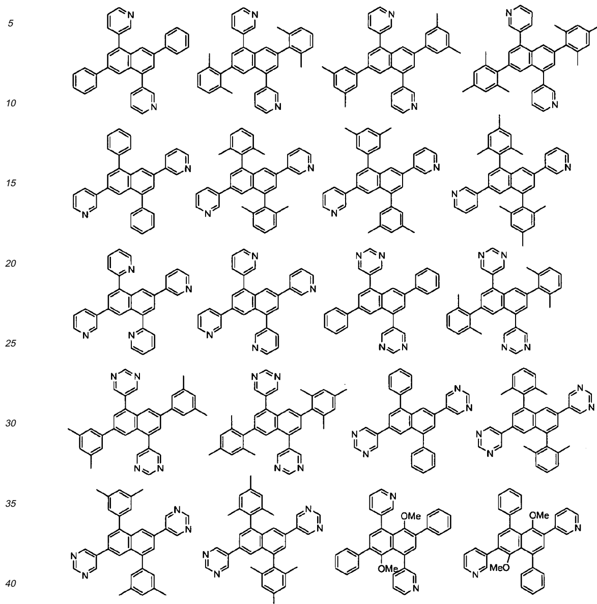
[Chemical Formula 8]
