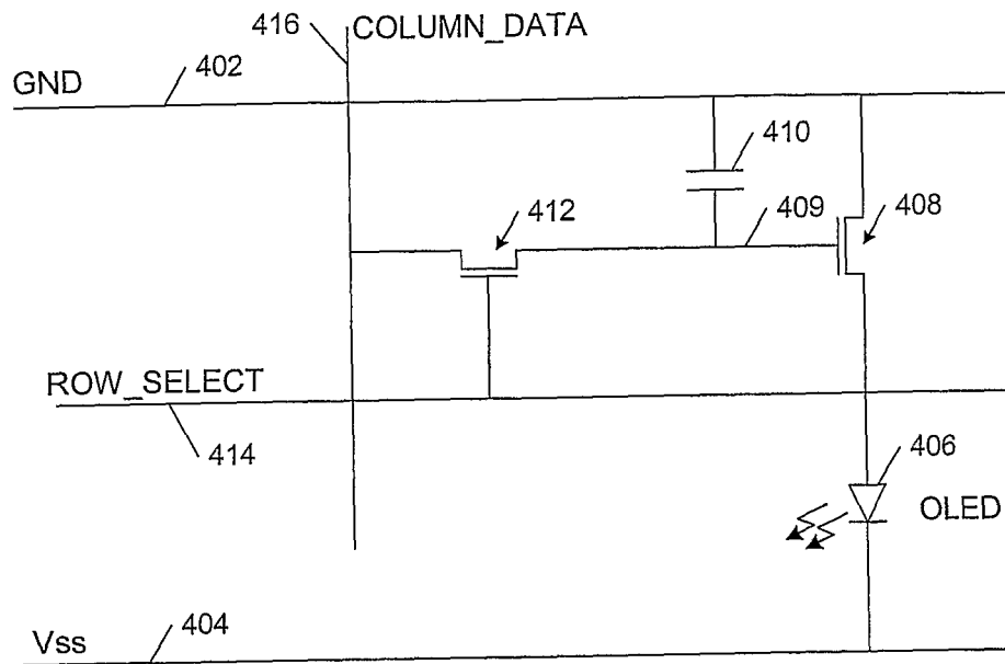
Figure 4 (PRIOR ART)
