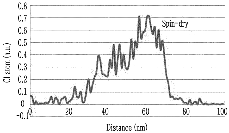
Cl distribution
