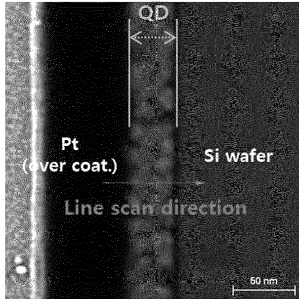
Cl distribution
