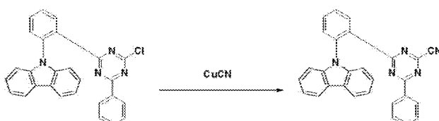
Compound 36
