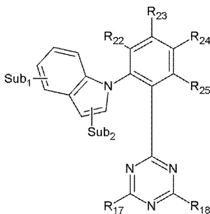
[Chemical Formula 10]
