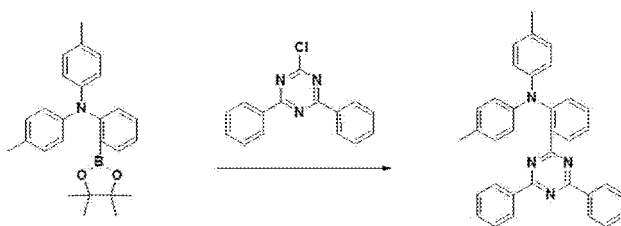
Compound 23
