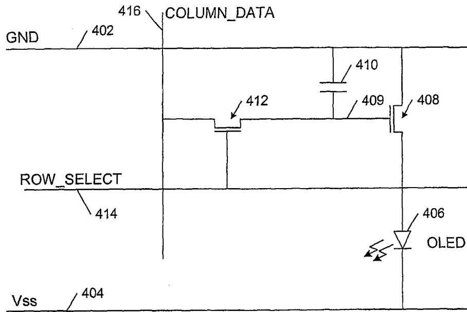
Figure 4 (PRIOR ART)
