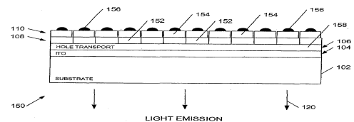
Figure 1b (PRIOR ART)
